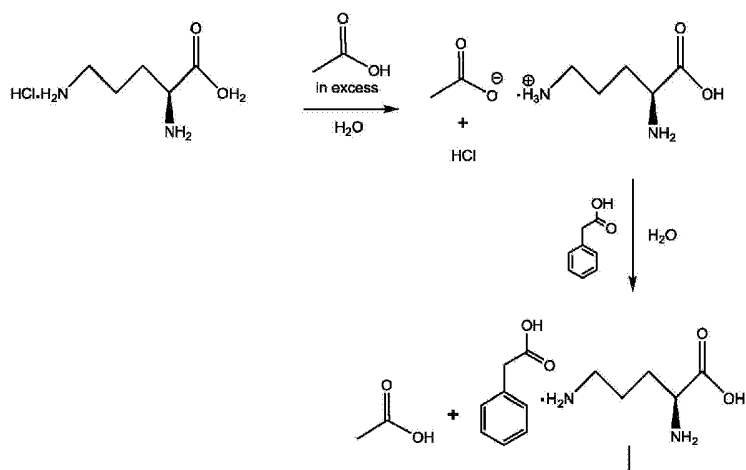
Scheme 3
