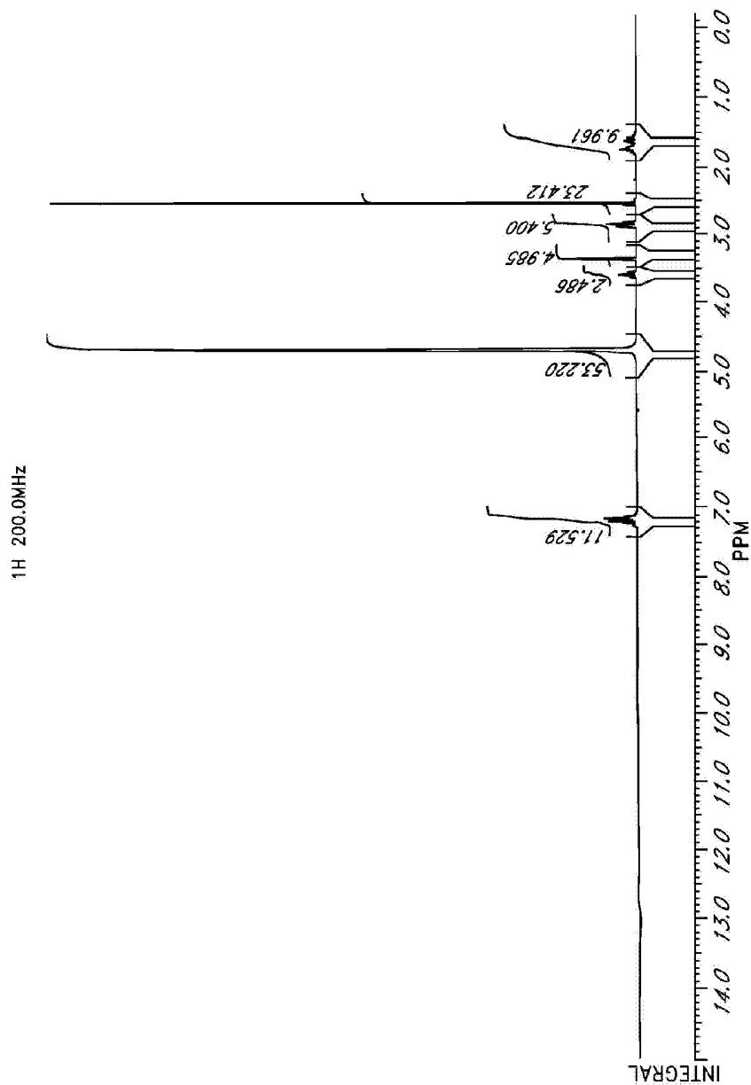
FIG. 22 Representative ^1\text{H} Spectra of L-ornithine phenyl acetate
