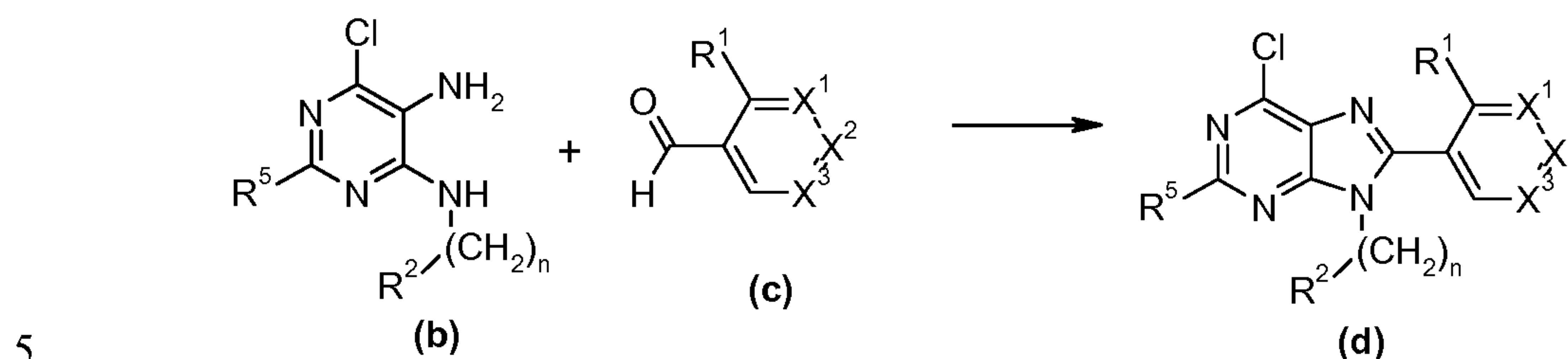
Scheme C
