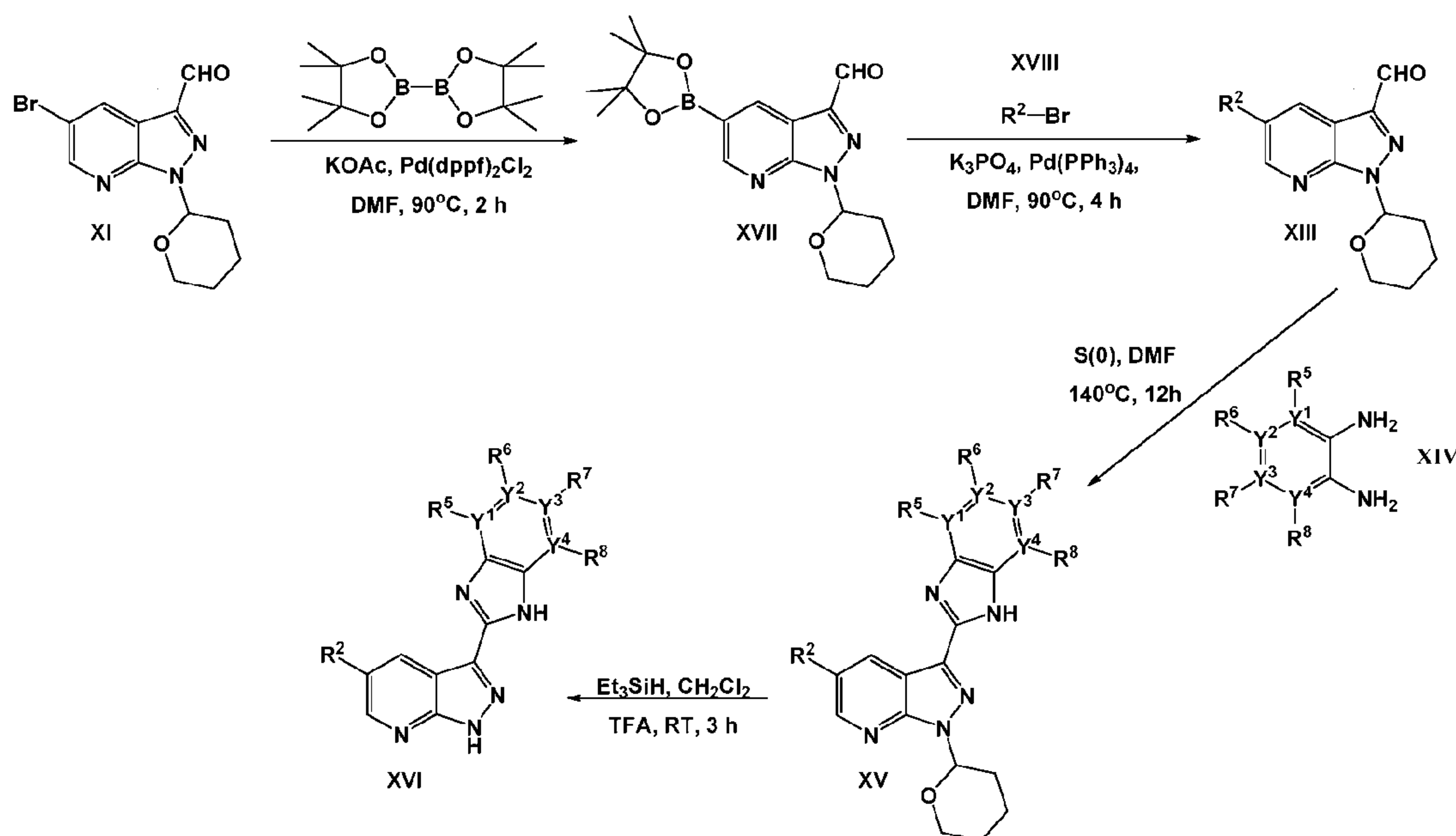
Scheme 2
