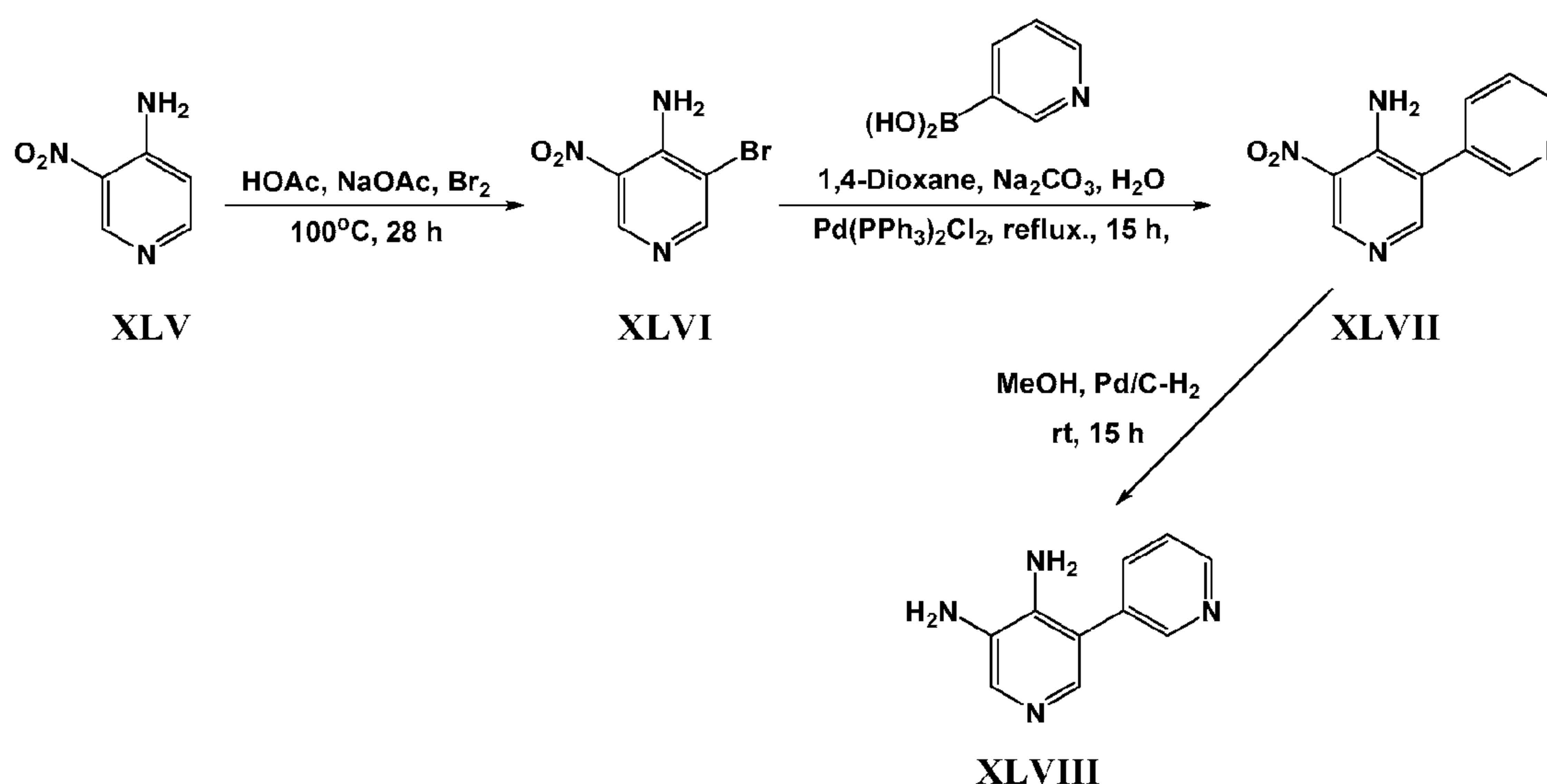
Scheme 8
