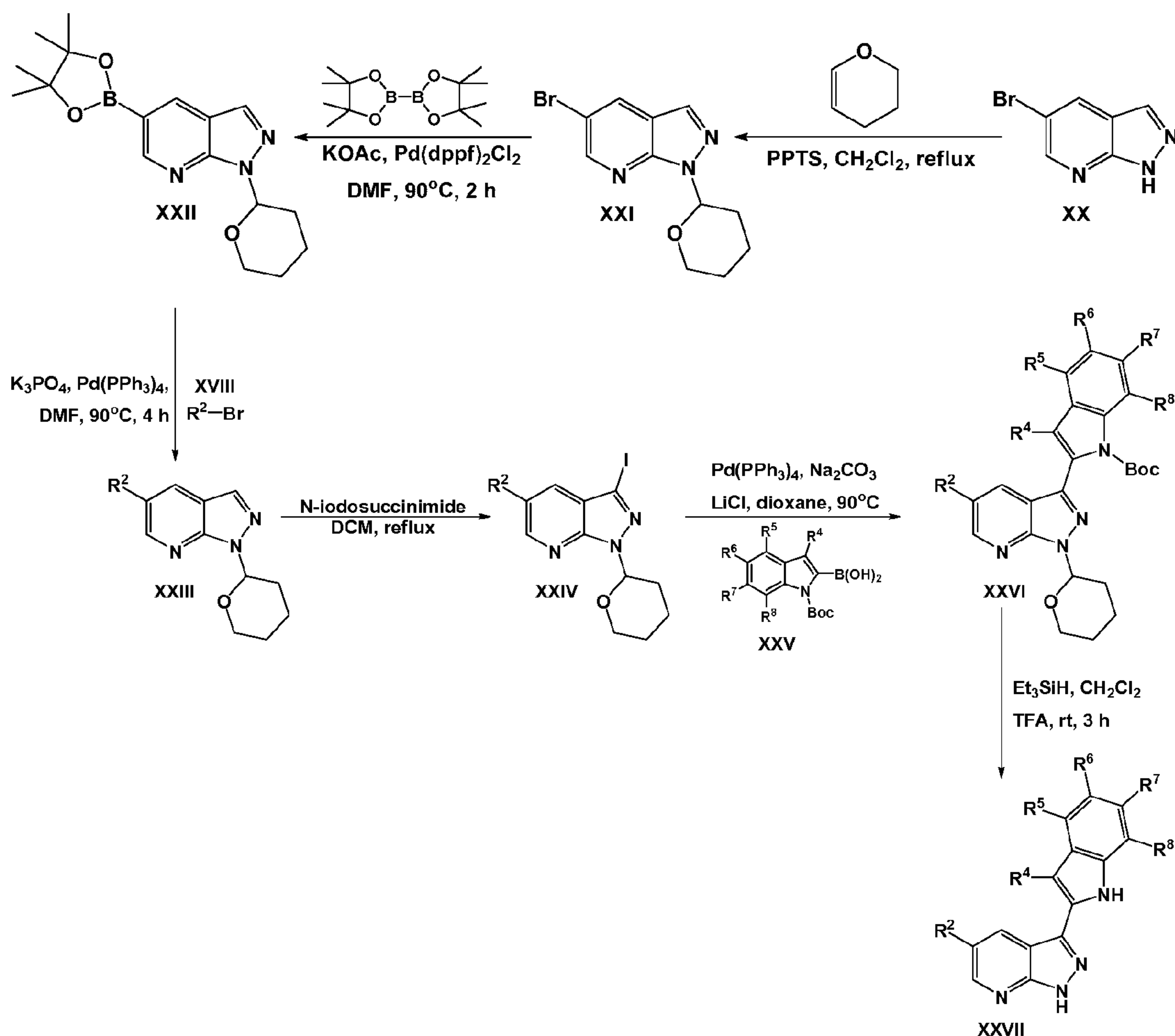
Scheme 3
