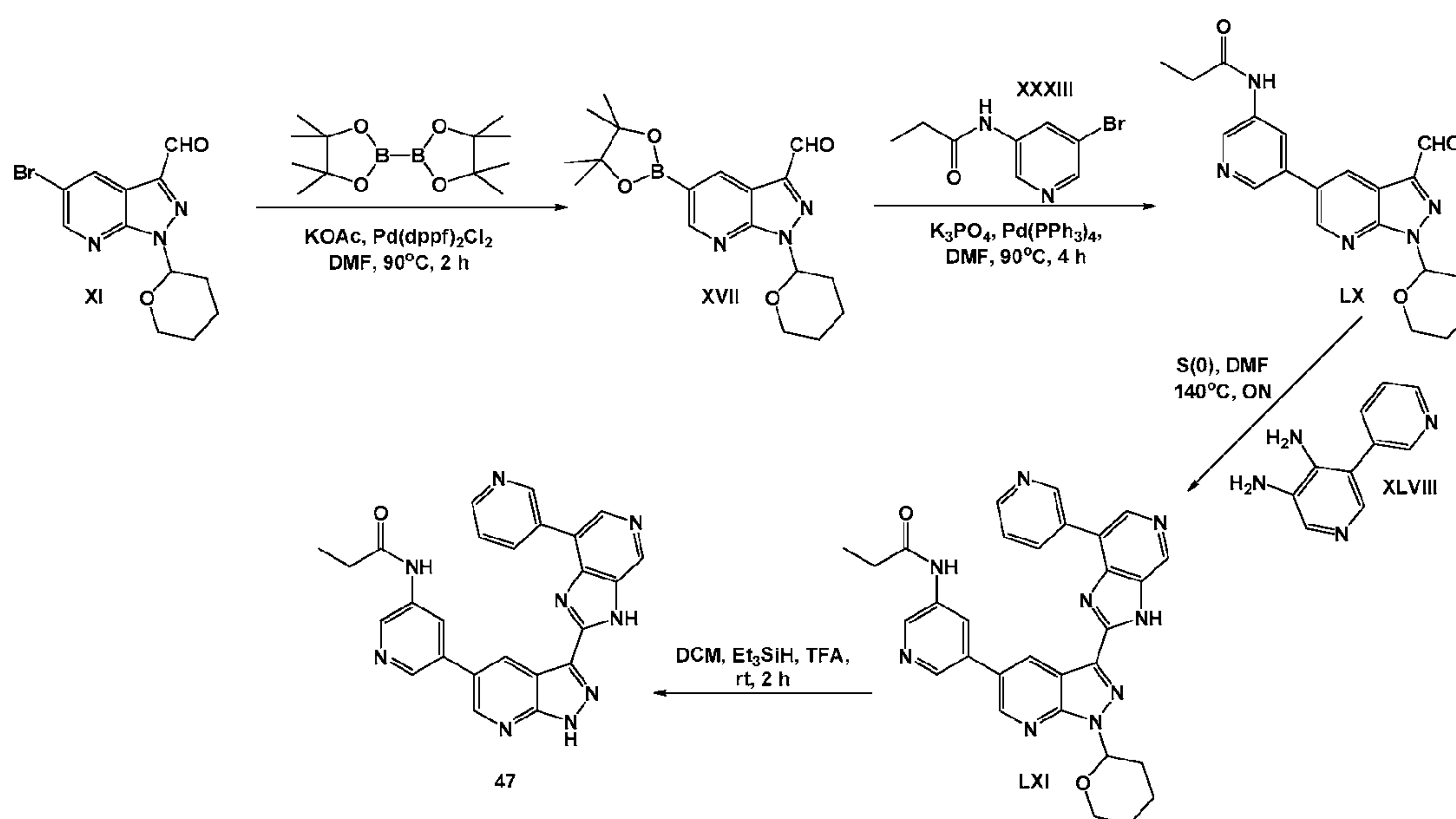
Scheme 11
