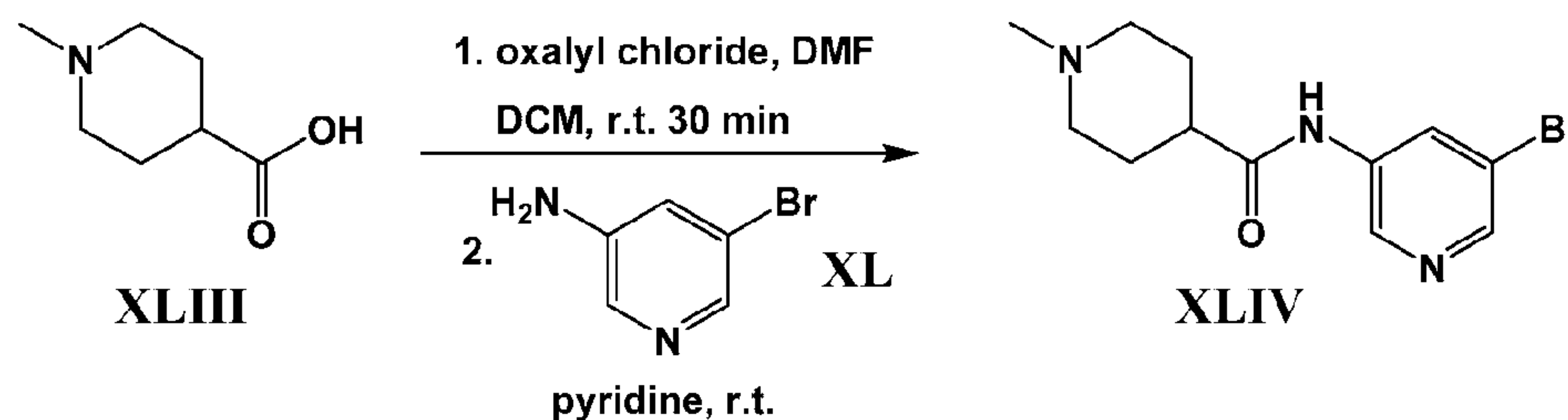
Scheme 7
