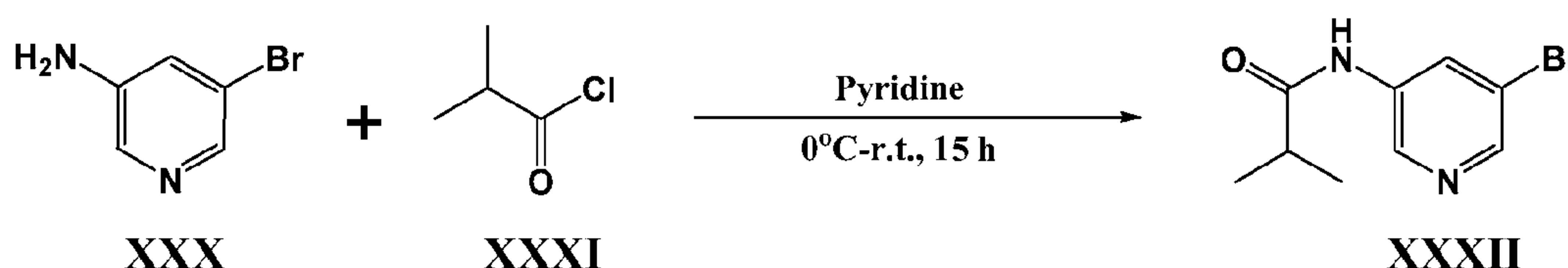
Scheme 5
