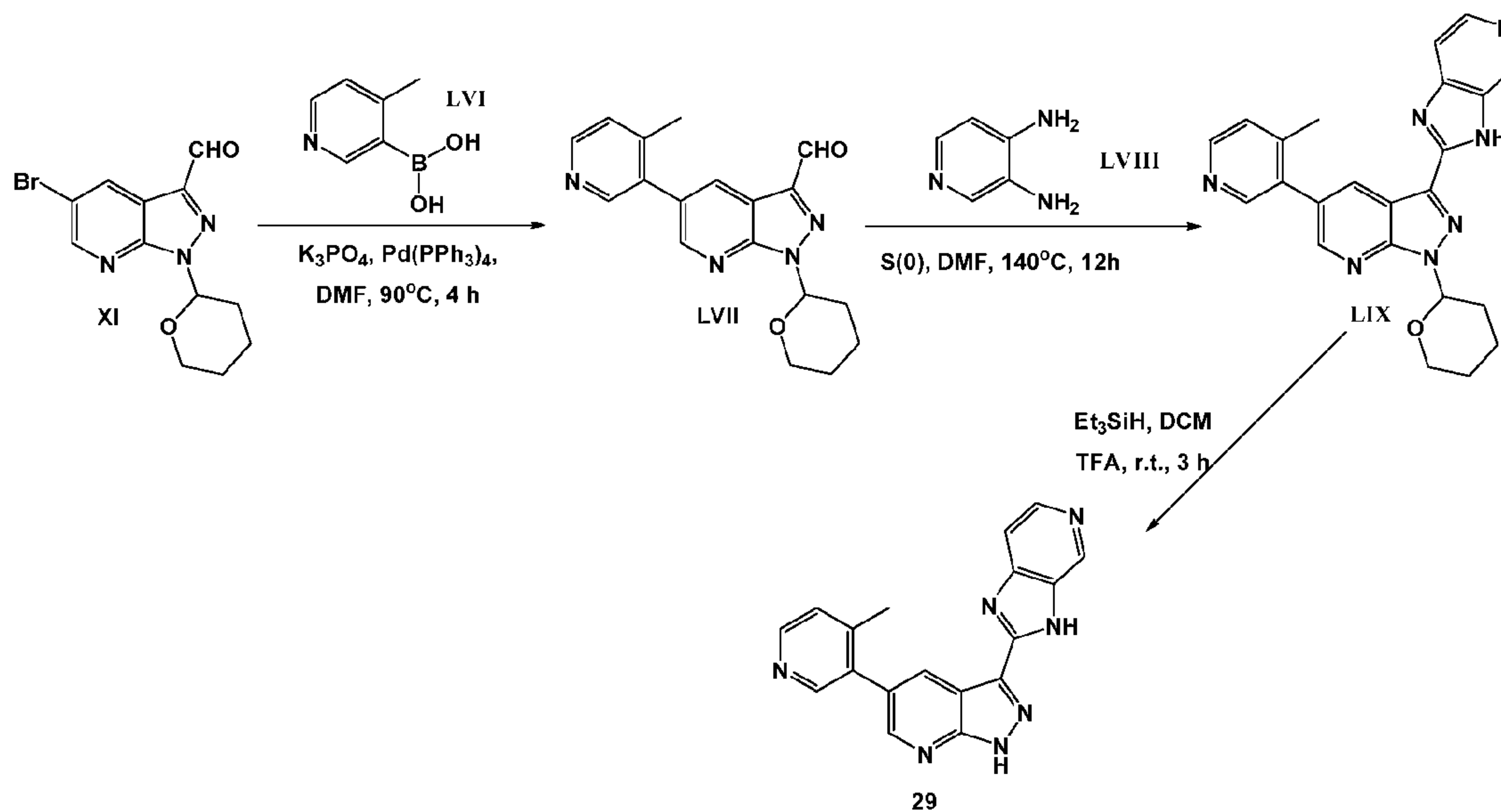
Scheme 10
