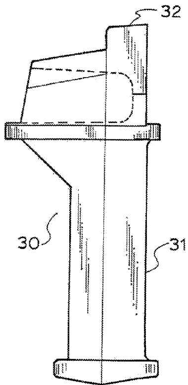
(PRIOR ART) Fig. 4
