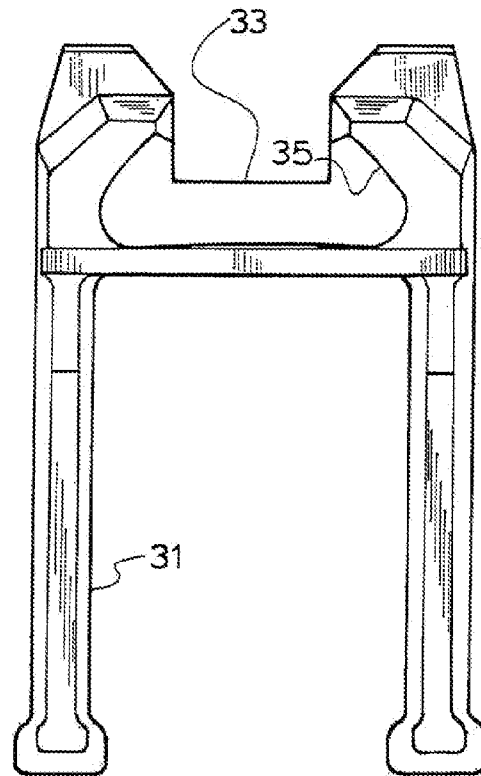
(PRIOR ART) Fig. 5
