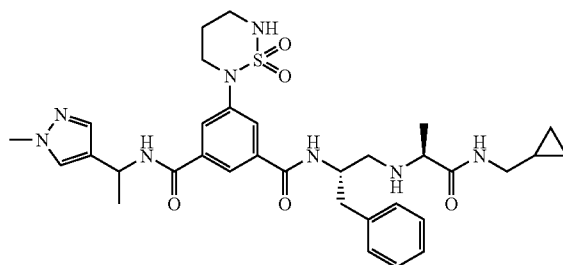
1-l
