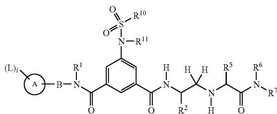
(Ic)
