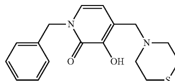
1-Benzyl-3-hydroxy-4-(thiomorpholin-4-ylmethyl)pyridin-2(1H)-one
