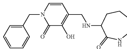
3-[(1-Benzyl-3-hydroxy-2-oxo-1,2-dihydropyridin-4-yl)methylamino]azepan-2-one
