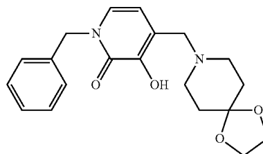
1-Benzyl-3-hydroxy-4-(1,4-dioxo-8-azaspiro[4,5]dec-8-ylmethyl)pyridin-2(1H)-one
