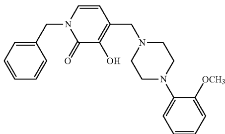
1-Benzyl-3-hydroxy-4-[4-(2-methoxyphenyl)piperazin-1-ylmethyl]pyridin-2(1H)-one
