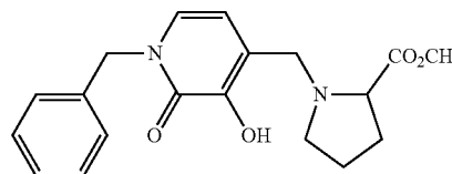
Methyl 1-[(1-benzyl-3-hydroxy-2-oxo-1,2-dihydropyridin-4-yl)methyl]pyrrolidine-2-carboxylate
