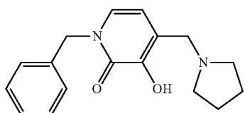
1-Benzyl-3-hydroxy-4-(pyrrolidin-1-ylmethyl)pyridin-2(1H)-one
