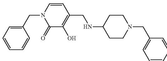
1-Benzyl-3-hydroxy-4-[(1-benzylpiperidin-4-ylamino)methyl]pyridin-2(1H)-one
