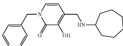
1-Benzyl-3-hydroxy-4-(cycloheptylaminomethyl)pyridin-2(1H)-one
