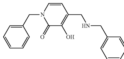
1-Benzyl-3-hydroxy-4-(benzylaminomethyl)pyridin-2(1H)-one
