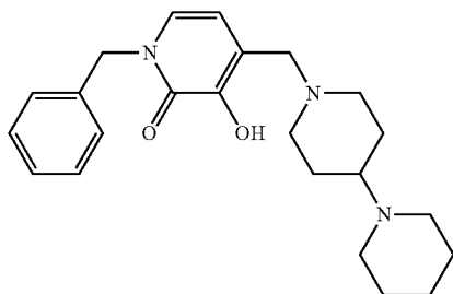
1-Benzyl-3-hydroxy-(1,4'-bipiperidinyl-1'-ylmethyl)pyridin-2(1H)-one
