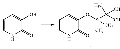
Scheme I
