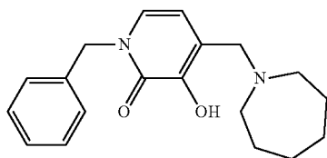
1-Benzyl-3-hydroxy-4-azepan-1-ylmethylpyridin-2-one (1H)-one
