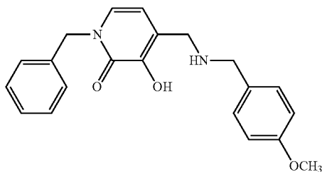
1-Benzyl-3-hydroxy-4-[(4-methoxybenzylamino)methyl]pyridin-2(1H)-one
