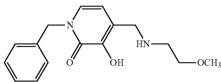
1-Benzyl-3-hydroxy-4-[(2-methoxyethyl)amino]methylpyridin-2(1H)-one
