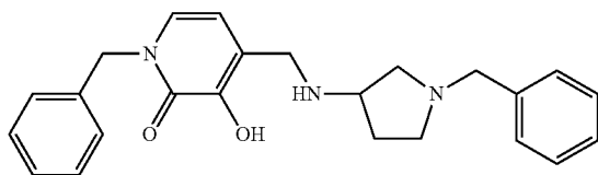
1-Benzyl-3-hydroxy-4-[(1-benzylpyrrolidin-3-ylamino)methyl]pyridin-2(1H)-one
