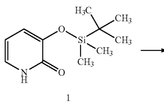
Scheme III
