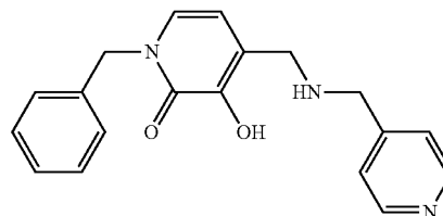
1-Benzyl-3-hydroxy-4-[(pyridin-4-ylmethyl)amino]methylpyridin-2(1H)-one
