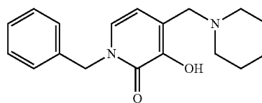
1-Benzyl-3-hydroxy-4-(piperidin-1-ylmethyl)pyridin-2(1H)-one
