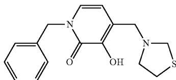
1-Benzyl-3-hydroxy-4-(thiazolidin-3-ylmethyl)pyridin-2(1H)-one
