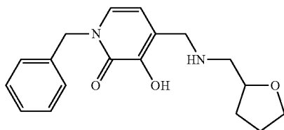
1-Benzyl-3-hydroxy-4-[(tetrahydrofuran-2-ylmethyl)amino]methylpyridin-2(1H)-one
