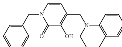
1-Benzyl-3-hydroxy-4-[(3,4-dihydroquinolin-1(2H)-yl)methyl]pyridin-2(1H)-one
