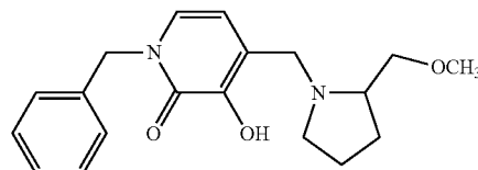
1-Benzyl-3-hydroxy-4-{[2-(methoxymethyl)pyrrolidin-1-yl]methyl}pyridin-2(1H)-one
