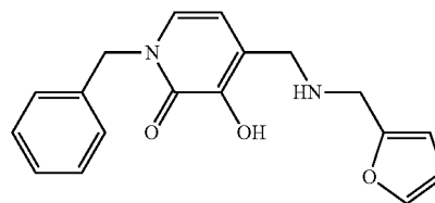
1-Benzyl-3-hydroxy-4-[(furan-2-ylmethyl)amino]methylpyridin-2(1H)-one
