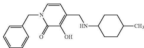
1-Benzyl-3-hydroxy-4-[(4-methylcyclohexylamino)methyl]pyridin-2(1H)-one
