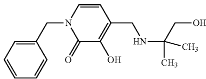
1-Benzyl-3-hydroxy-4-[(1-hydroxy-2-methylpropan-2-yl)amino]methylpyridin-2(1H)-one
