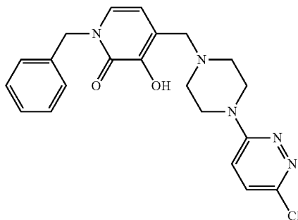
1-Benzyl-3-hydroxy-4-[4-(6-chloropyridazin-3-yl)piperazin-1-ylmethyl]pyridin-2(1H)-one
