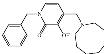
1-Benzyl-3-hydroxy-4-(azocan-1-ylmethyl)pyridin-2-one (1H)-one
