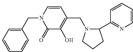
1-Benzyl-3-hydroxy-4-([2-(pyridin-2-yl)pyrrolidin-1-yl]methyl)pyridin-2(1H)-one
