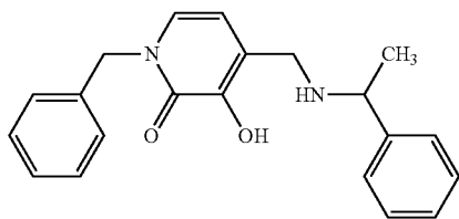
1-Benzyl-3-hydroxy-4-[(1-phenylethylamino)methyl]pyridin-2(1H)-one
