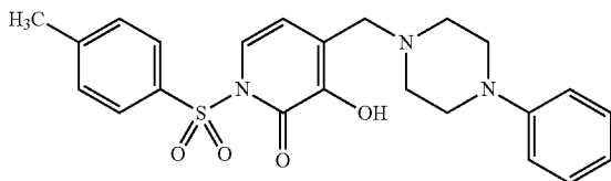
1-(4-Methylbenzenesulfonyl)-3-hydroxy-4-(4-phenylpiperazin-1-ylmethyl)-pyridin-2(1H)-one
