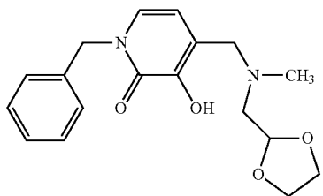
1-Benzyl-3-hydroxy-4-[(1,3-dioxolan-2-ylmethyl)ethylamino]methyl]pyridin-2(1H)-one
