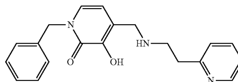
1-Benzyl-3-hydroxy-4-{[2-(pyridin-2-yl)ethylamino]methyl}pyridin-2(1H)-one
