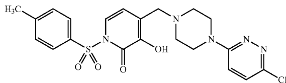
1-(4-Methylbenzenesulfonyl)-3-hydroxy-4-[4-(6-chloropyridazin-3-yl)piperazin-1-ylmethyl]pyridin-2(1H)-one
