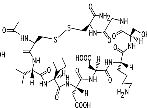
N-Ac-CVIDDKSGC-NH 2
