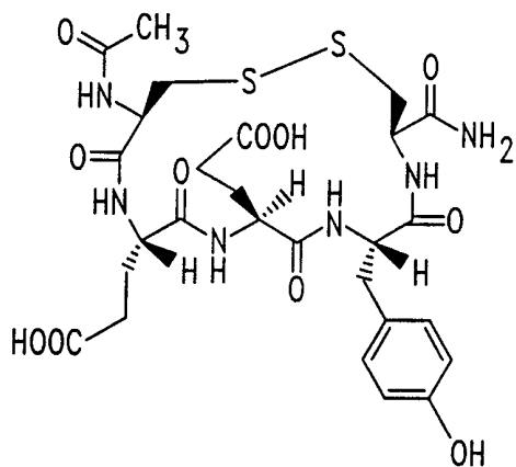
N-Ac-CEEYC-NH 2
