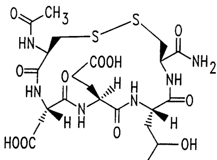
N-Ac-CDETC-NH 2
