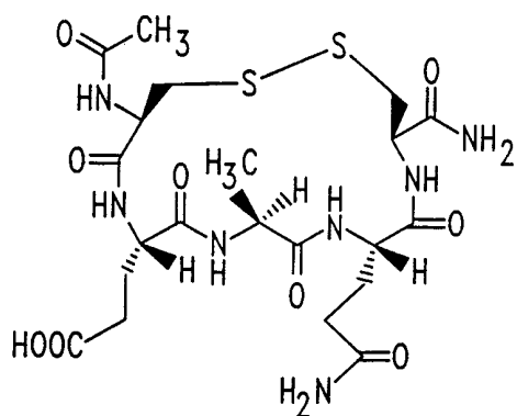
N-Ac-CEAQC-NH 2
