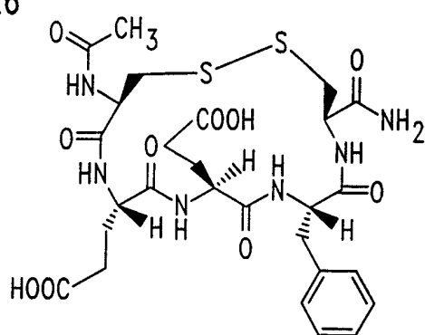
N-Ac-CEEFC-NH 2
