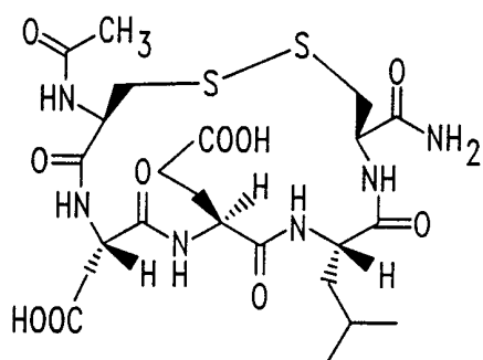
N-Ac-CDELC-NH 2
