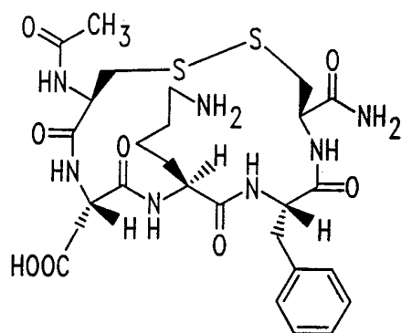
N-Ac-CDKFC-NH 2
