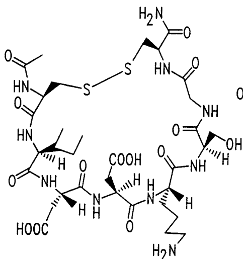
N-Ac-CIDDKSGC-NH 2
