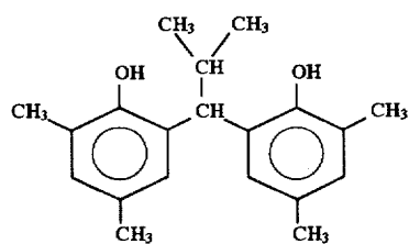
(Cpd-310) Fungicide
