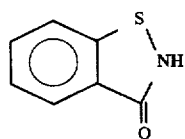
(Cpd-311) Fungicide
