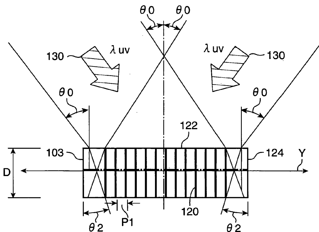
PRIOR ART FIG. 10B
