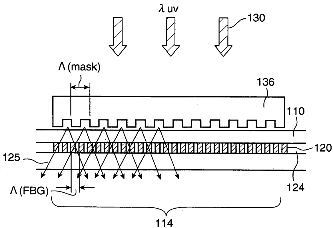
PRIOR ART FIG. 12
