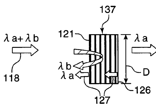
PRIOR ART FIG. 10C
