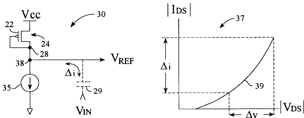
FIG. 5 (Prior Art)
