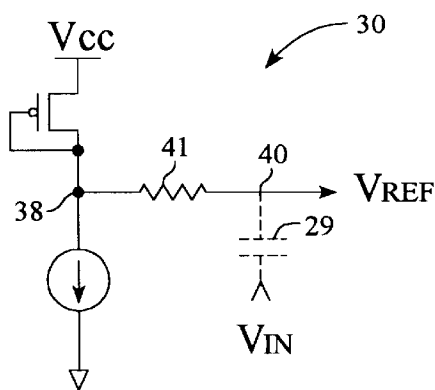
FIG. 6 (Prior Art)
