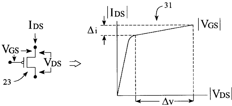
FIG. 3 (Prior Art)
