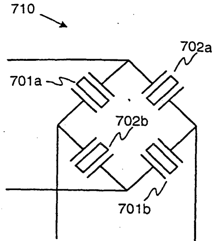
Fig. 7b PRIOR ART
