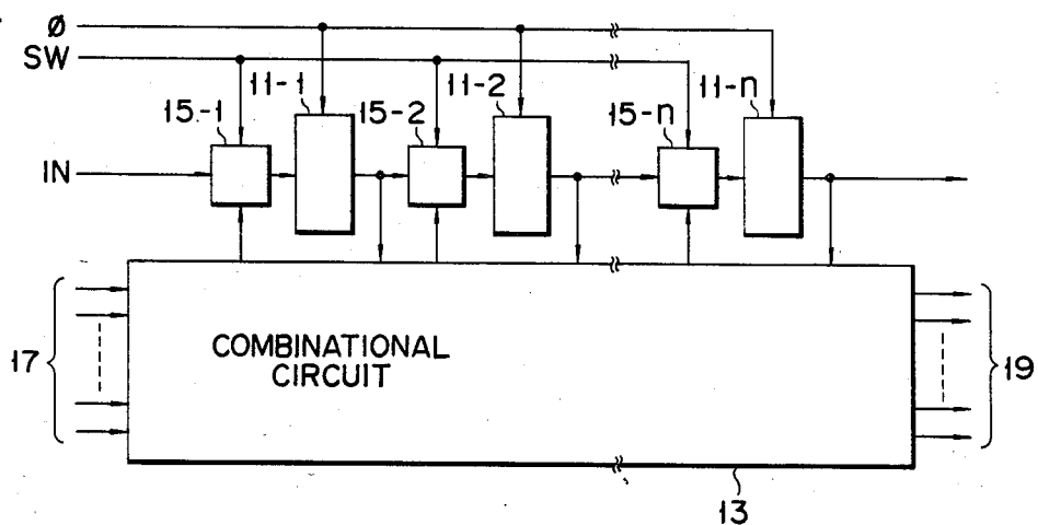
FIG. 2 (PRIOR ART)
