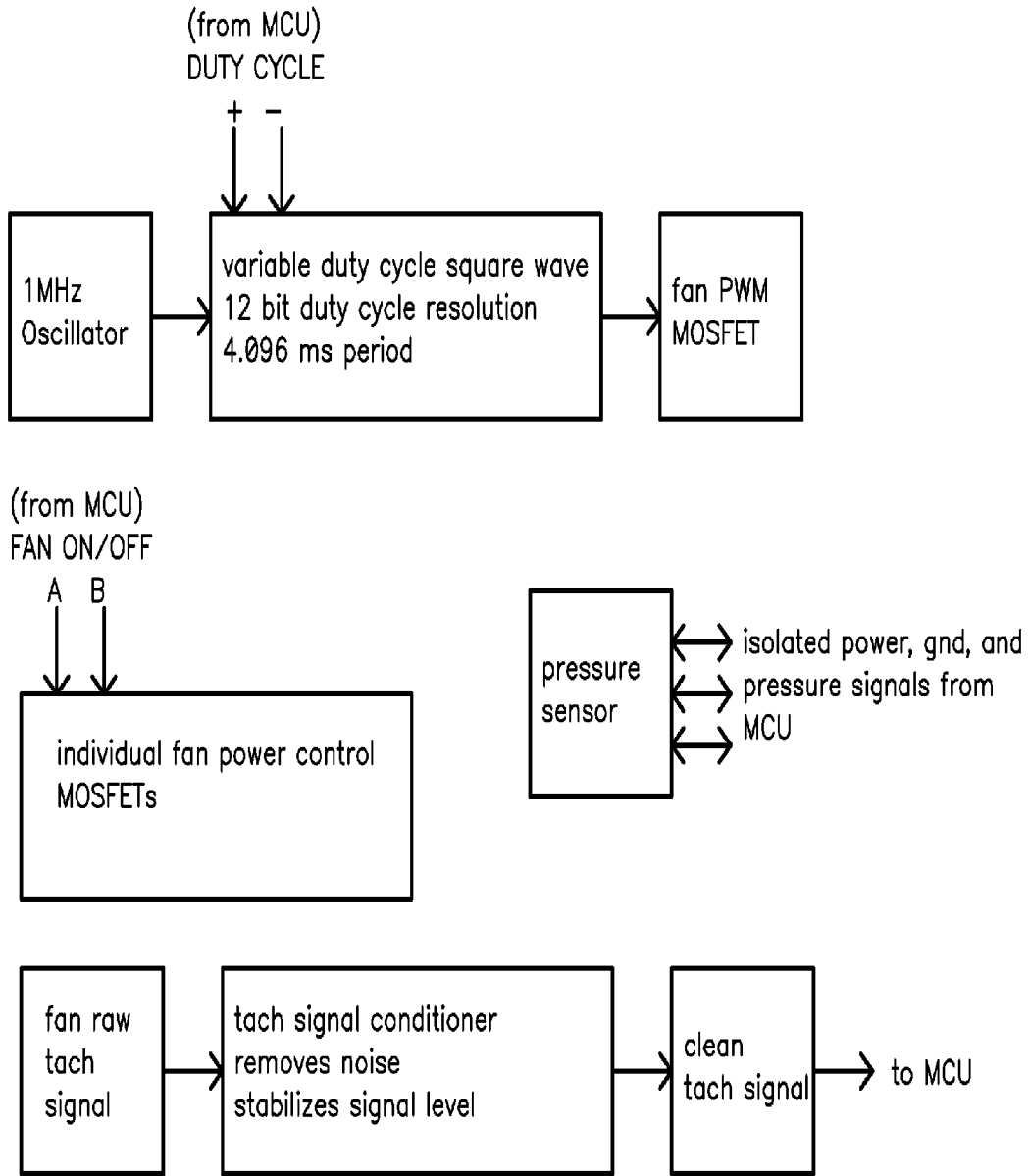
BLOWER CONTROL SYSTEM PWM PCB FUNCTIONAL DIAGRAM
