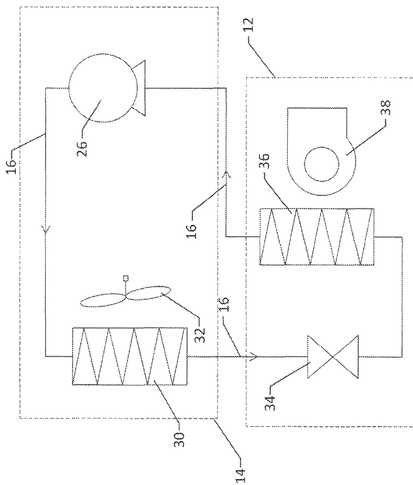
FIG. 3 (PRIOR ART)
