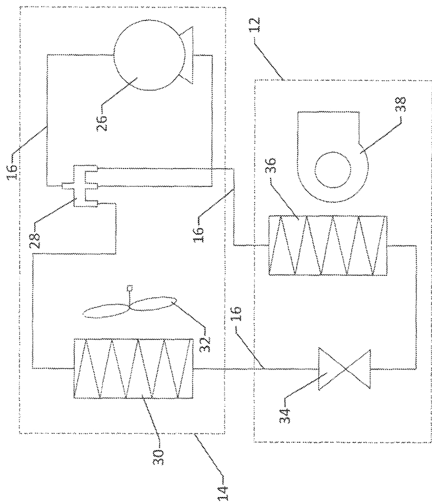
FIG. 2 (PRIOR ART)
