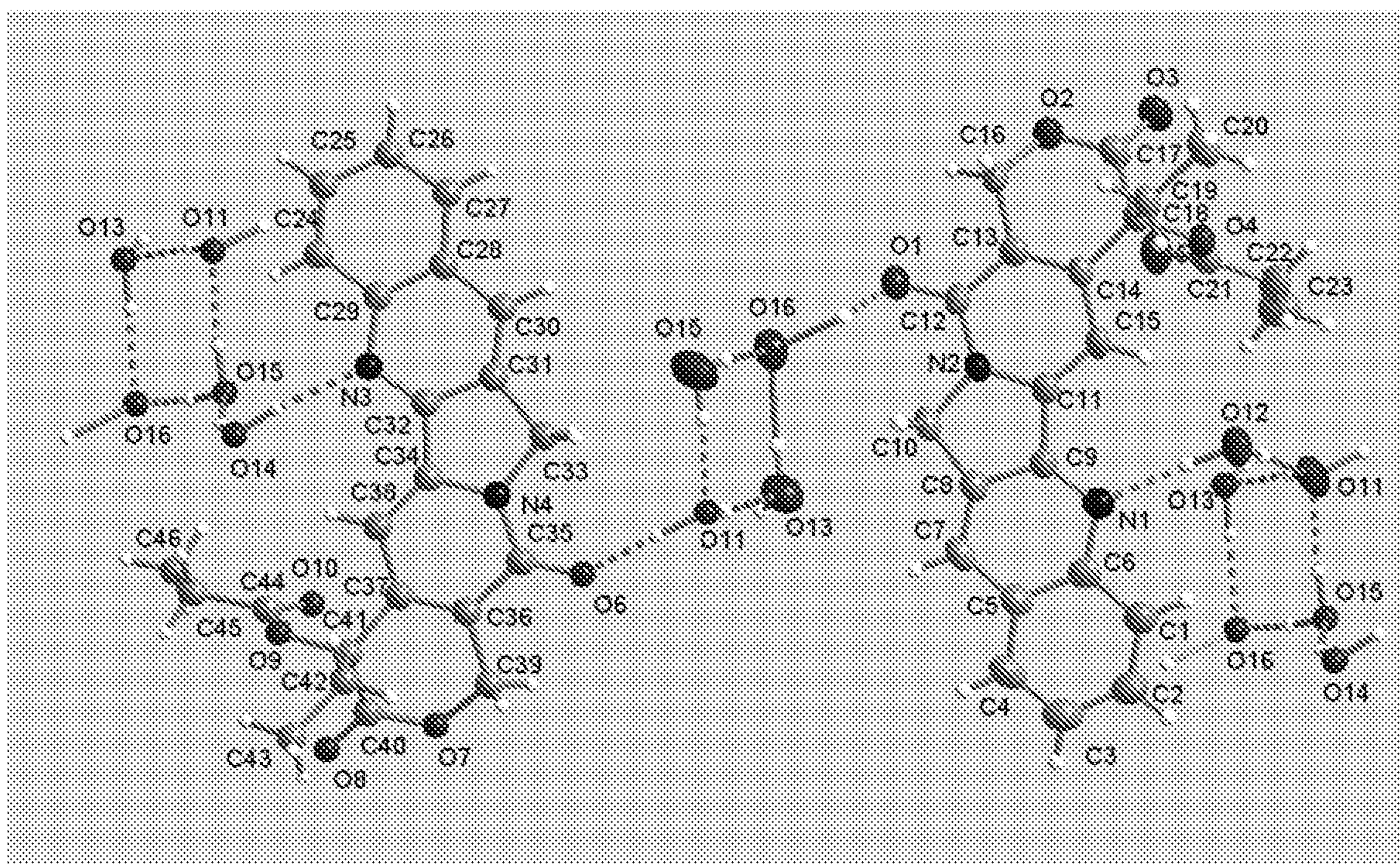
Fig. 2. H 2 O bridged Molecular Structure of 2 x C 23 H 20 N 2 O 5 ·3H 2 O
