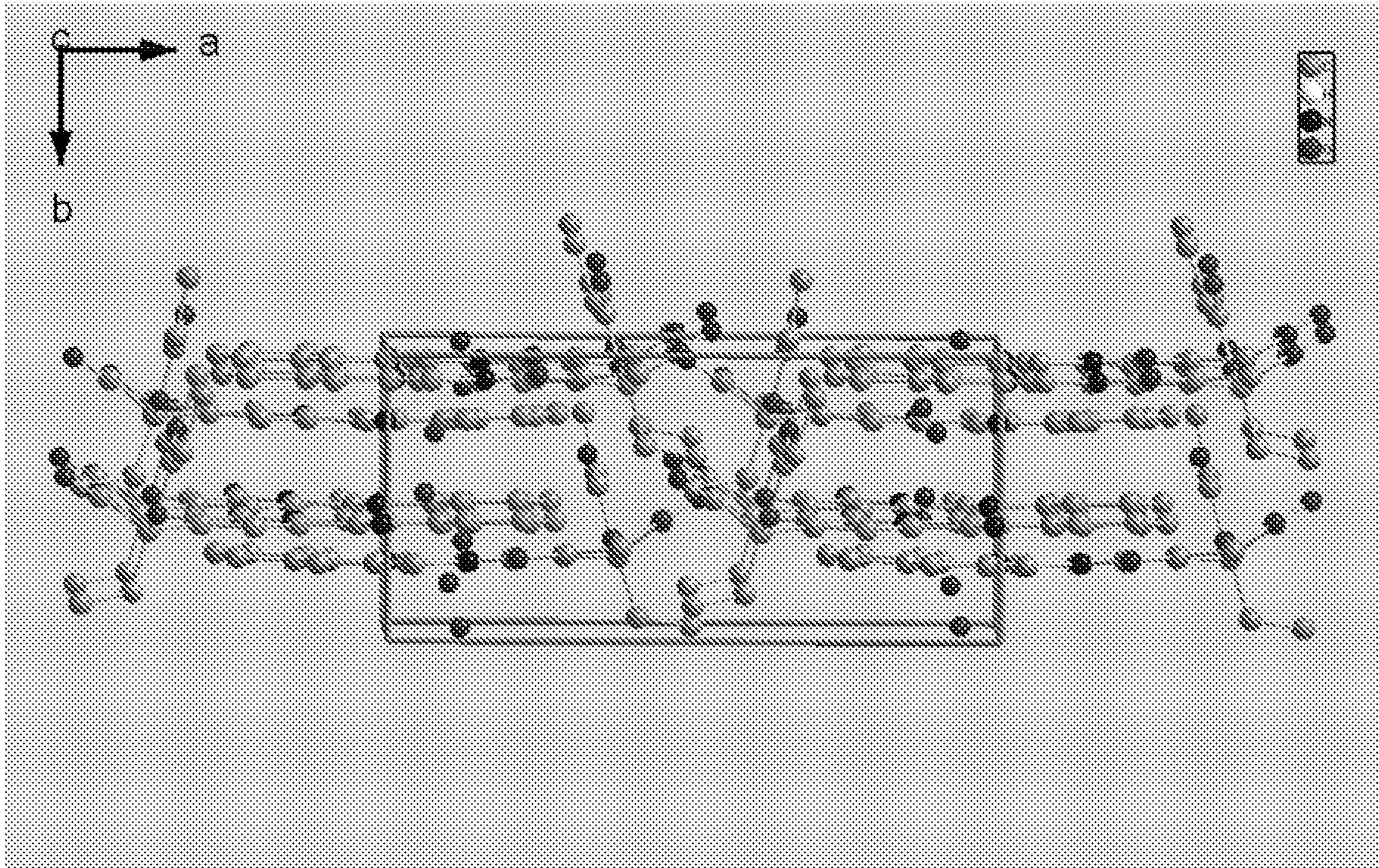
Fig. 3. Three Dimentional Crystal Structure of C_{23}H_{20}N_2O_5 \cdot 3H_2O ( a,b -dimentions)
