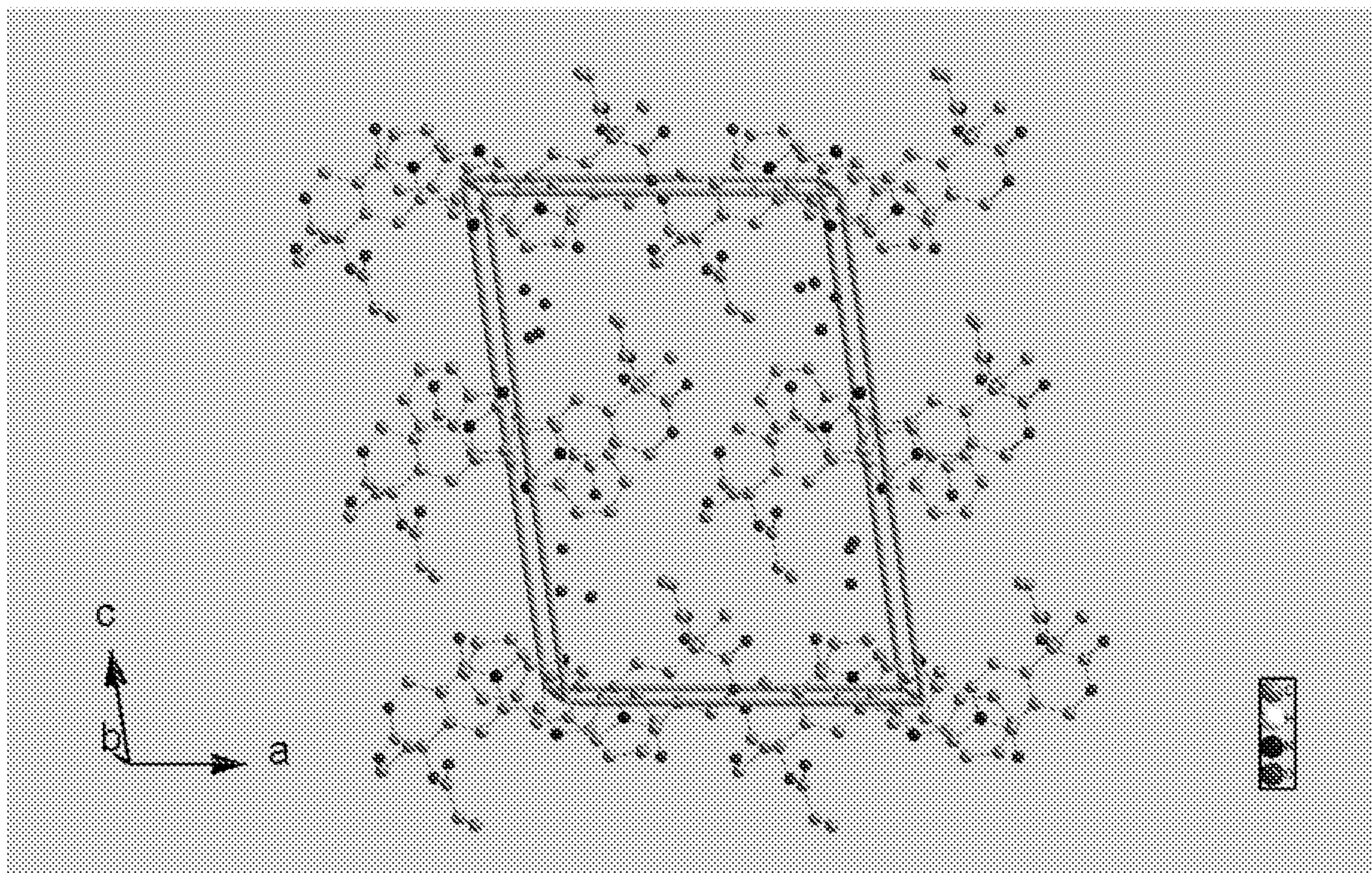
Fig. 4. Three Dimensional Crystal Structure of C_{23}H_{20}N_2O_5 \cdot 3H_2O (a,c-dimensions)
