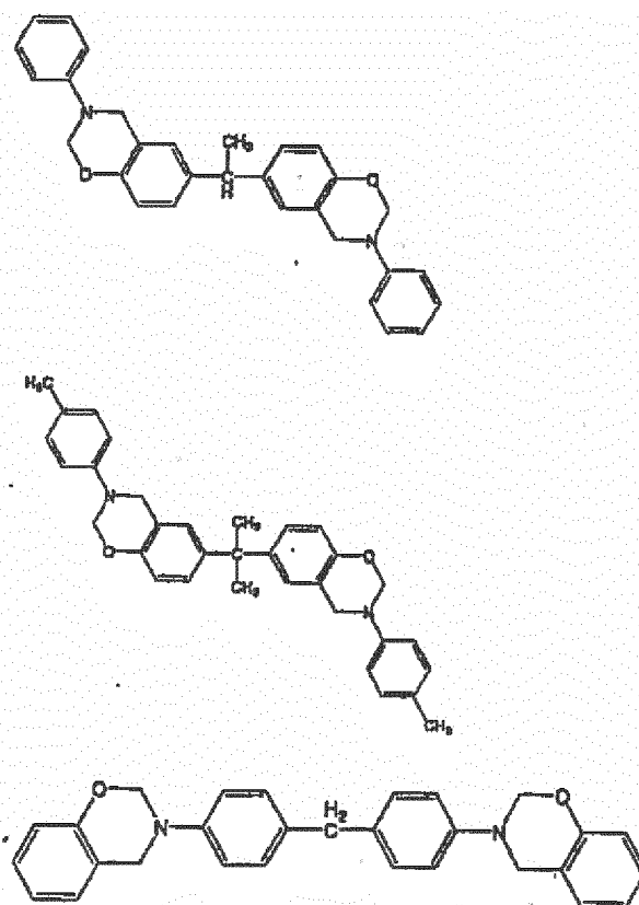
[Chemical Formula 9]
