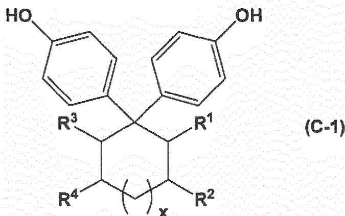
[Chemical Formula 1]
