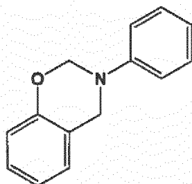
[Chemical Formula 9]
