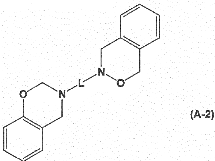
[Chemical Formula 5]
