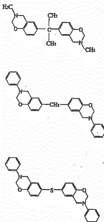
[Chemical Formula 6]
