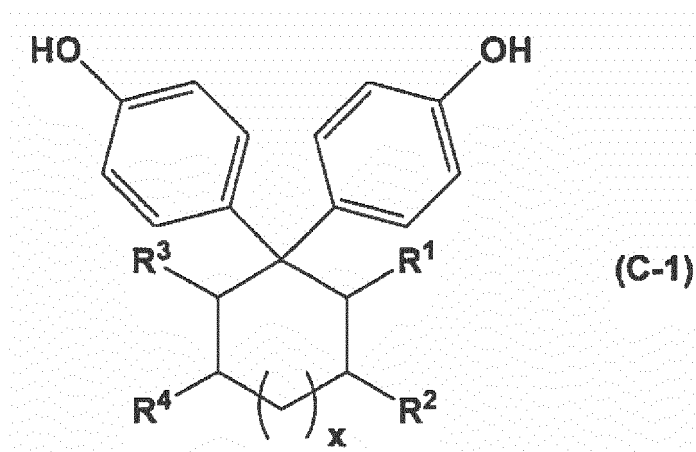
[Chemical Formula 2]
