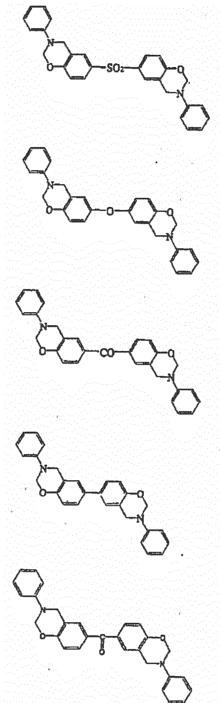
[Chemical Formula 8]
