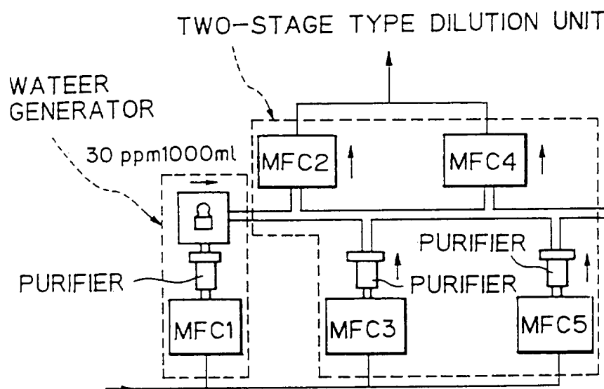
SCHEMATIC LAYOUT FOR GENERATION AND DILUTION OF STANDARD GAS OF LOW WATER CONTENT
