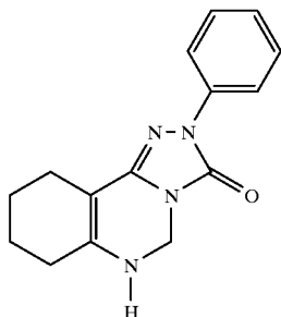
Compound 31
