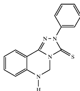
Compound 29
