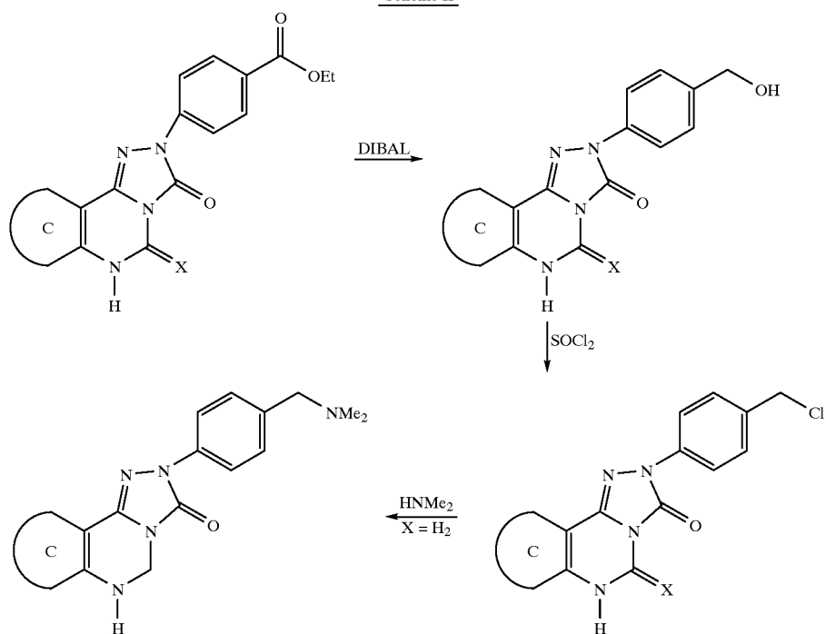
Scheme II
