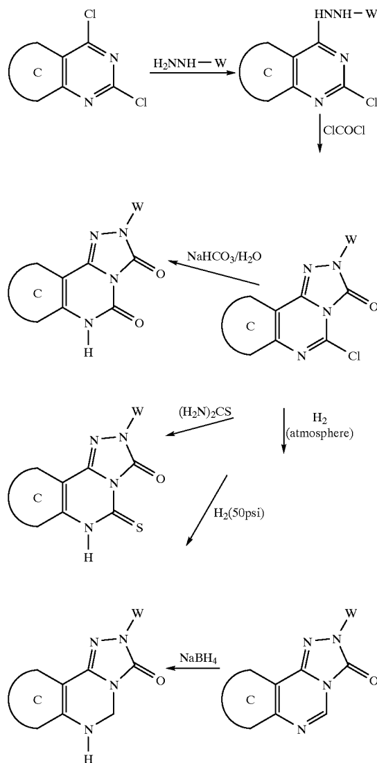
Scheme I
