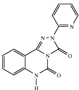
Compound 5
