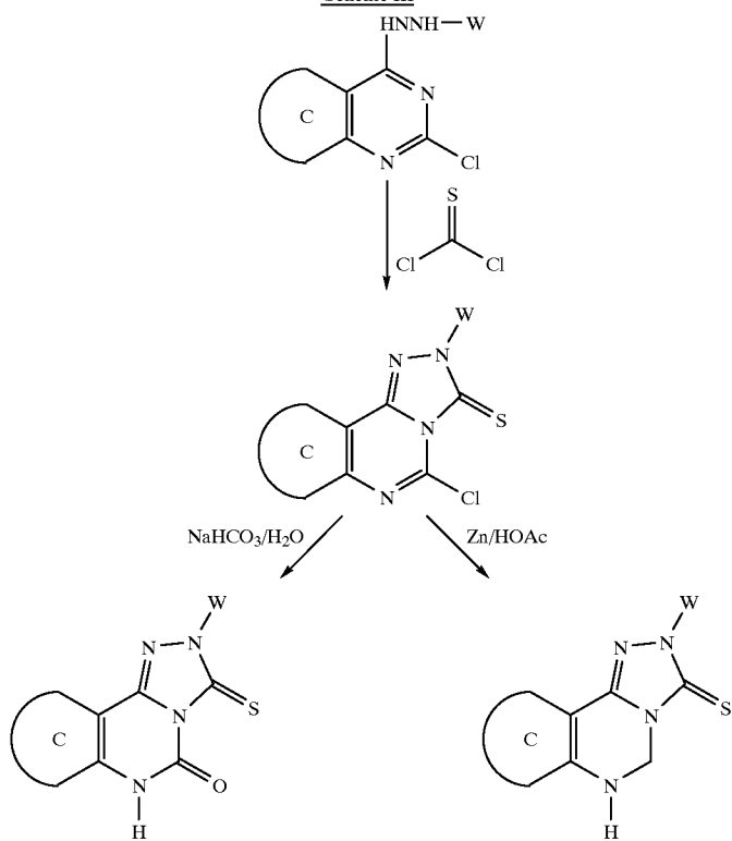
Scheme III
