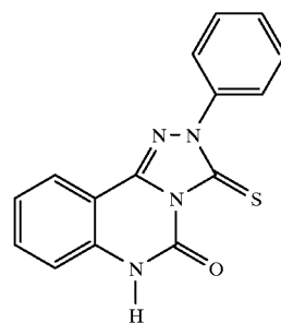
Compound 28
