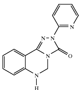
Compound 13
