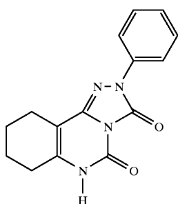
Compound 30
