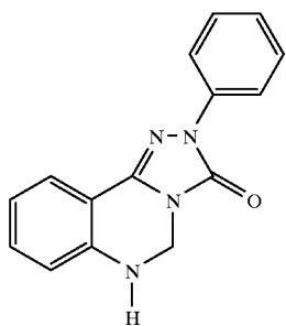
Compound 2
