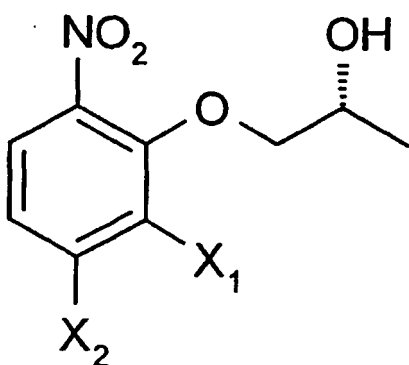
generic formula 2
