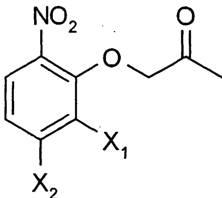
generic formula 1
