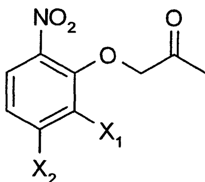
generic formula 1
