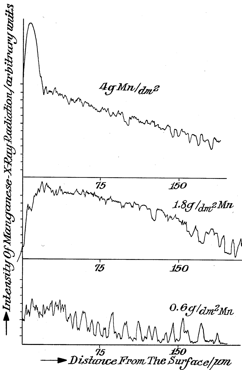
Fig. 2. Manganese Profile Of Manganized Titanium Sheet.
