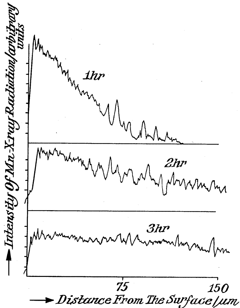
Fig. 1. Manganese Profile Of Manganized Titanium Sheet, Manganese Layer: 2\text{g}\cdot\text{dm}^{-2} Temperature: 950^{\circ}\text{C} . Annealing Period Under Vacuum 1, 2 or 3 Hours Surface Concentration Of Mn: 60, 45 and 30 % (estimated)
