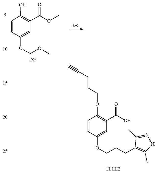
SCHEME 3. Synthesis of TLHE2.
