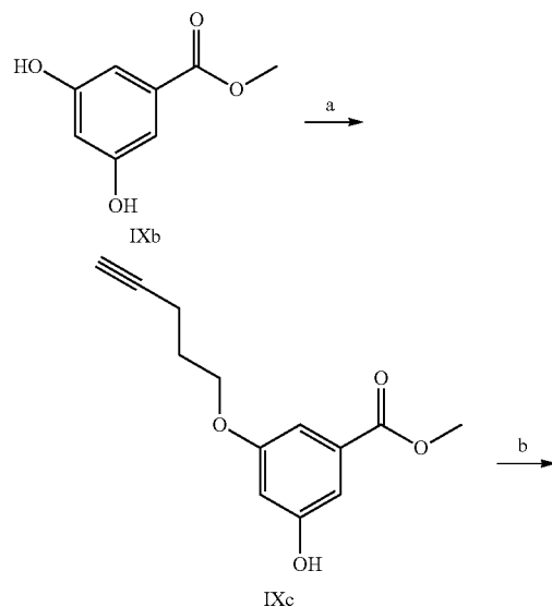
SCHEME 2. Synthesis of TLHE1.
