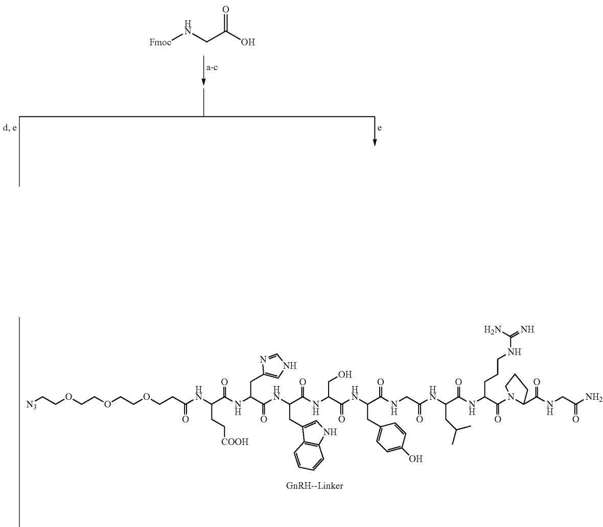
SCHEME 6. Synthesis of GnRH-Linker, and Conj3.
