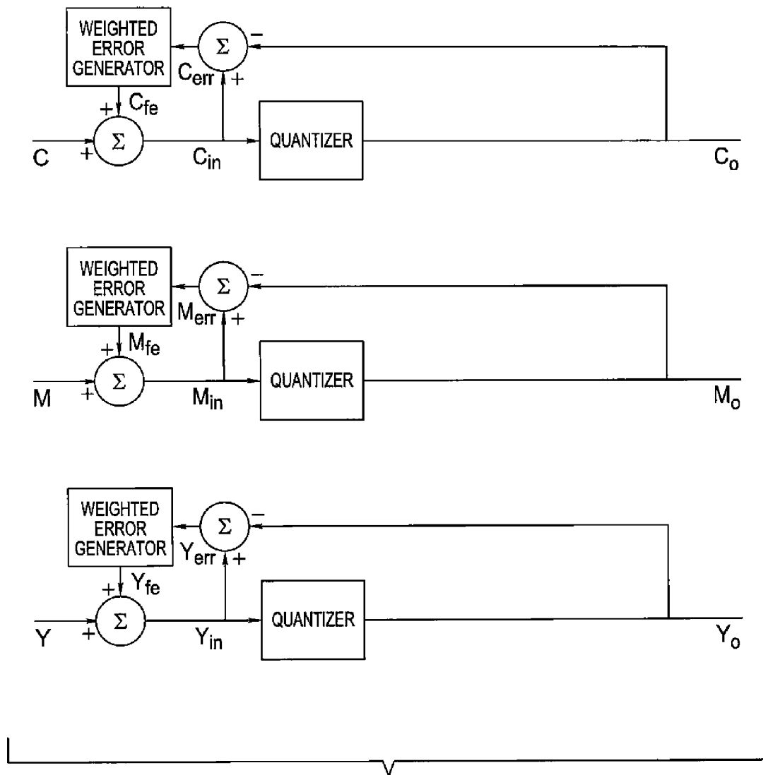
FIG. 3 PRIOR ART
