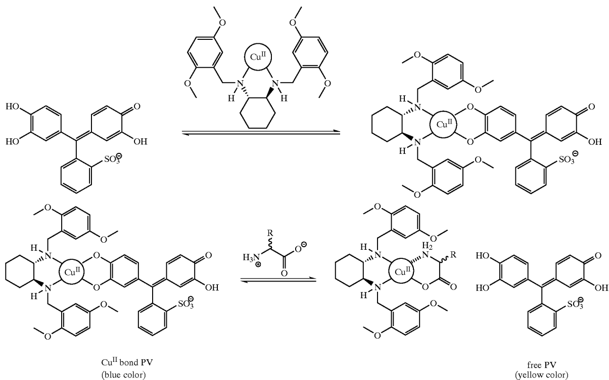
Scheme S-24. The Indicator Displacement Process Being Monitored in Scheme S-23.
