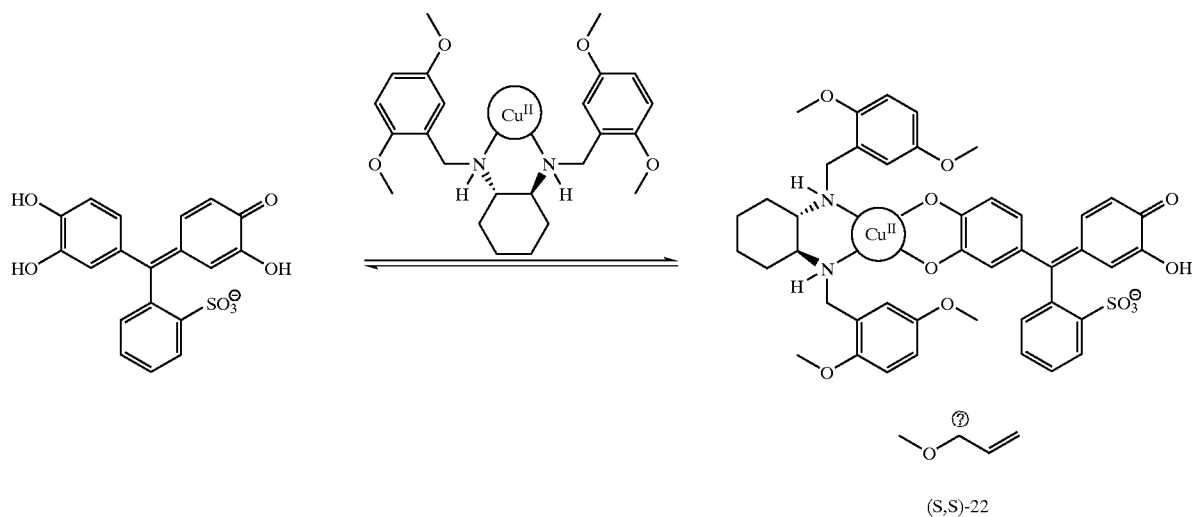
Scheme S-22. Synthesis of (S,S)-22 by Reductive Amination.
