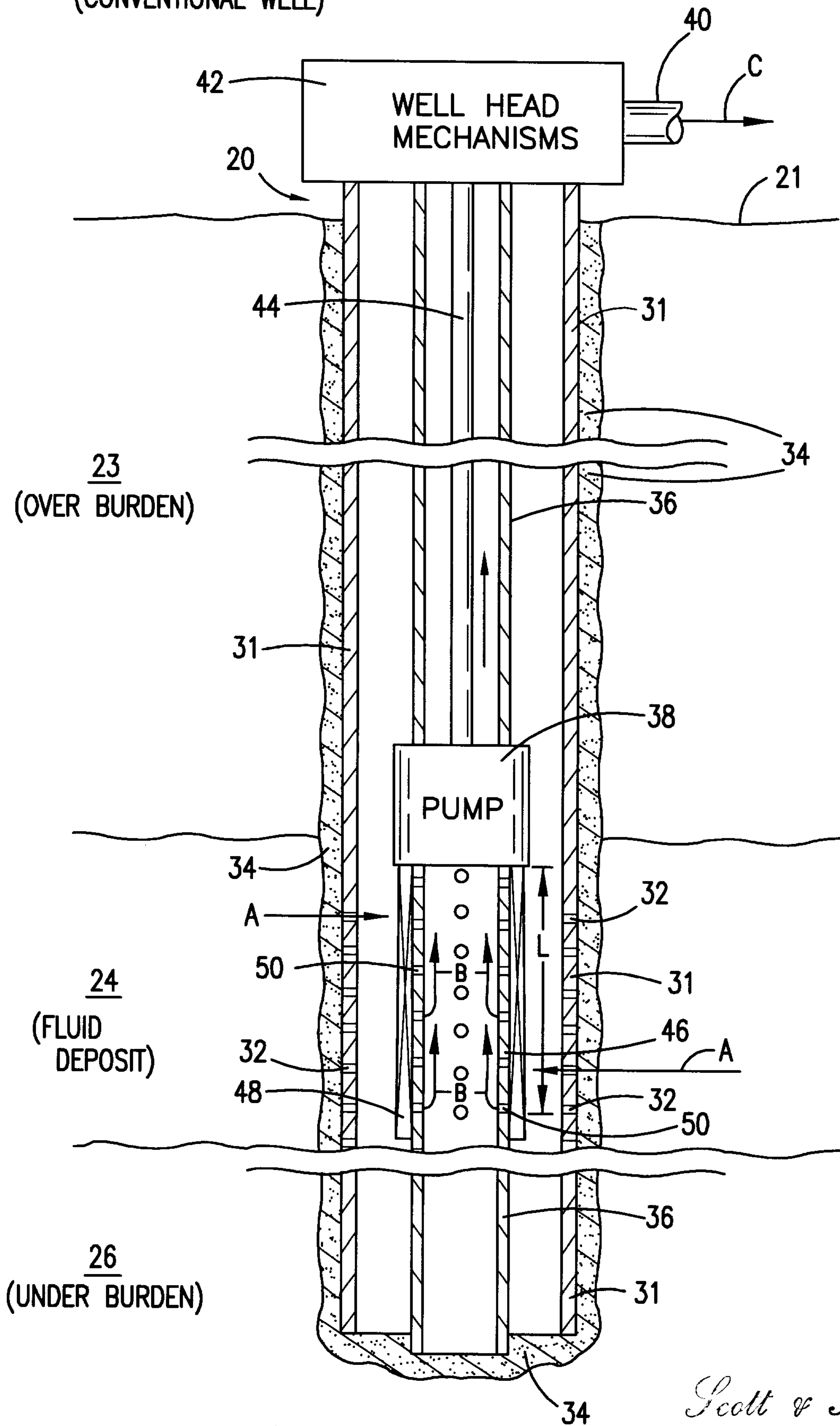
FIG. 1 (CONVENTIONAL WELL)
