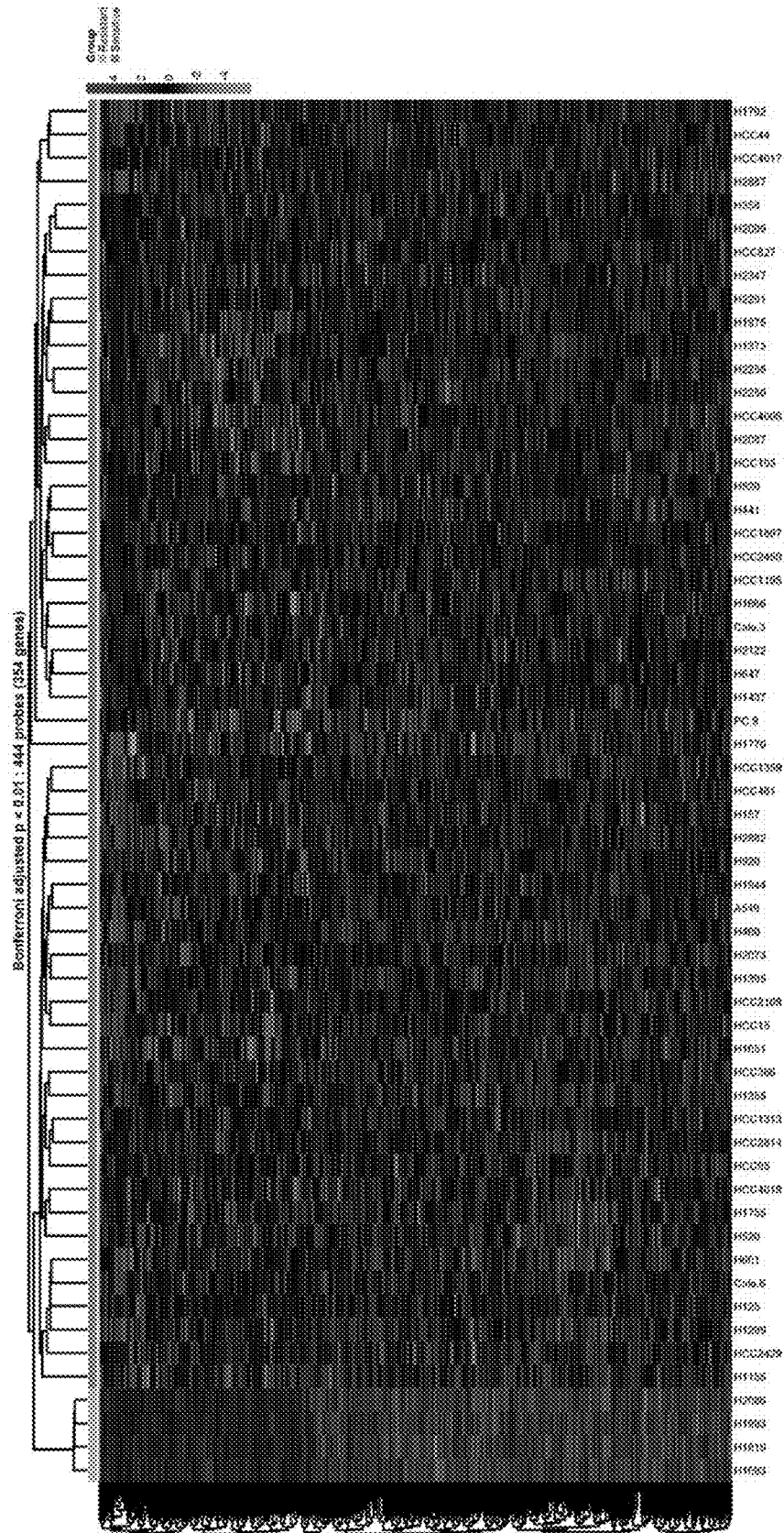
FIG. 15 Cluster Analysis Adding Another 6-thio-dG Resistant Cell Line Improved the Separation of 6-thio-dG Resistant NSCLC from Sensitive NSCLC Cell Lines
