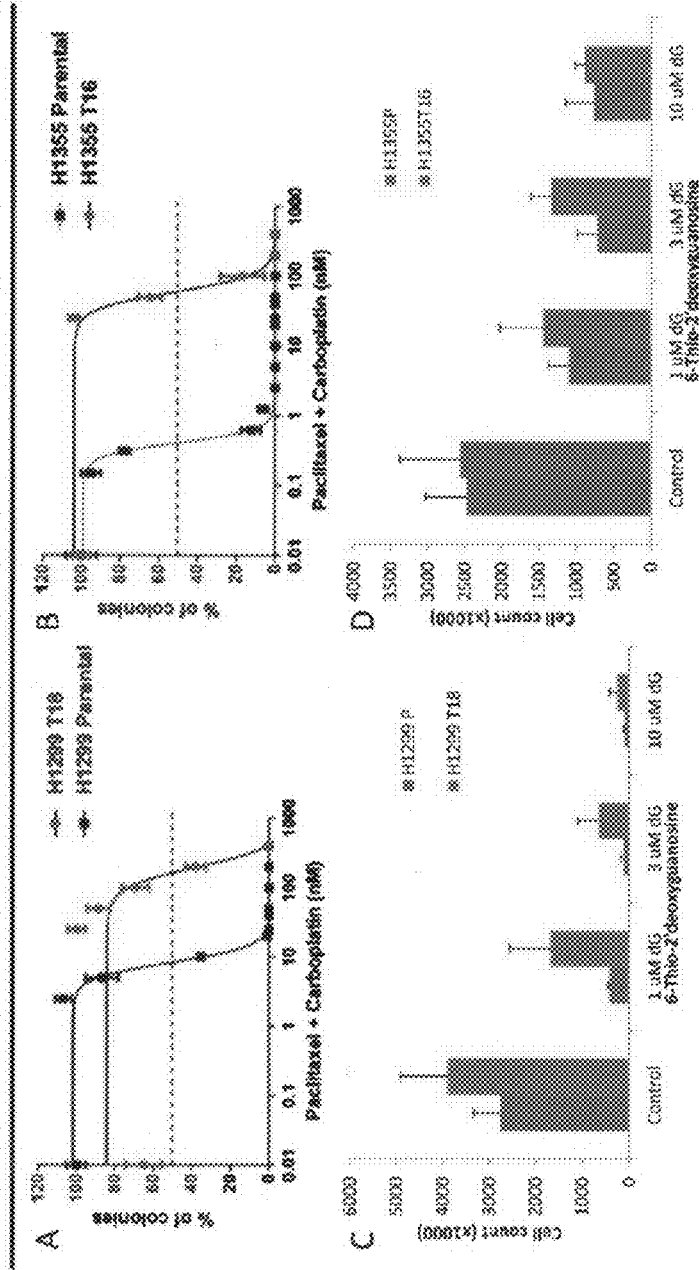
FIG. 16 Paclitaxel-Carboplatin Resistant H1299 and H1355 NSCLC is Sensitive to 6-thio-dG
