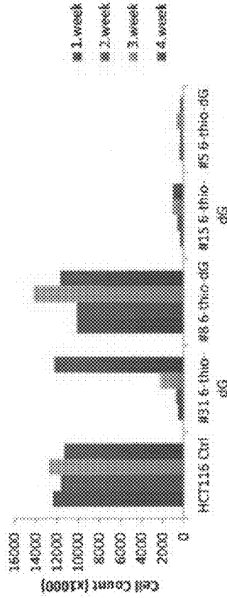
Selected HCT116 Clones for Cell Count
