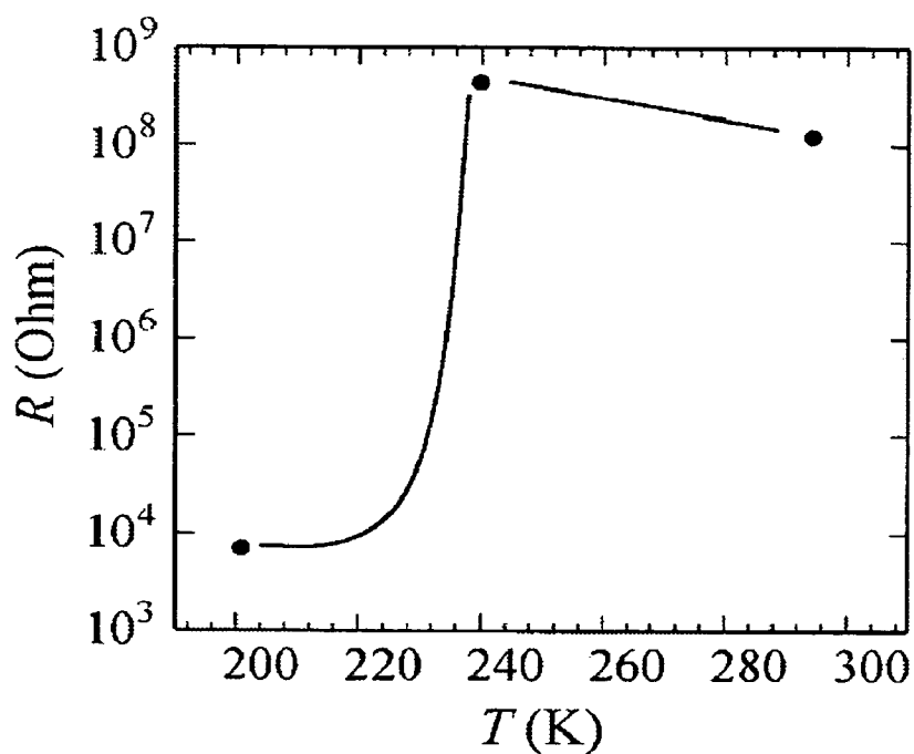
Resistance-Temperature Curve of Hetero Junction ( V=-3V )
