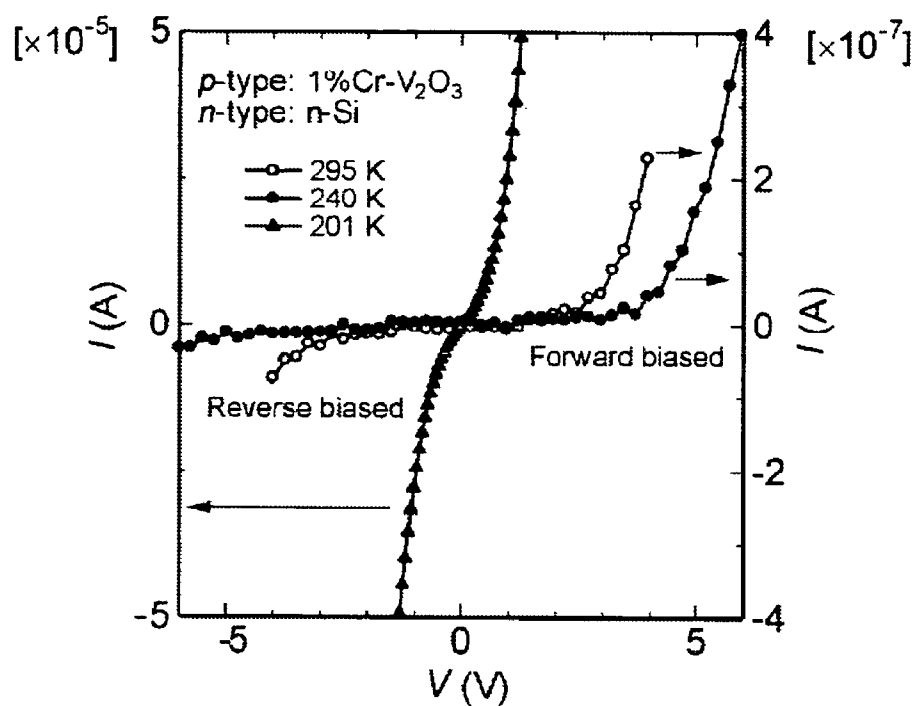
I-V characteristics of the hetero junction
