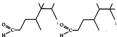
FIG. 7 is the NMR spectrum for the diisoundecanal compounds produced according to Example II having the structures:
