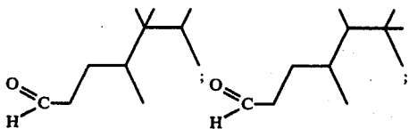
FIG. 8 is the infra-red spectrum for the diisoundecanal compounds produced according to Example II having the structures:
