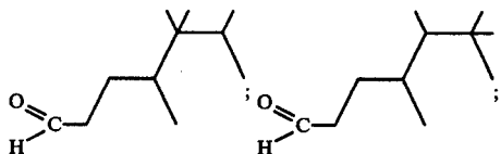
FIG. 6 is the GLC profile for the diisoundecanal compounds produced according to Example II having the structures:
