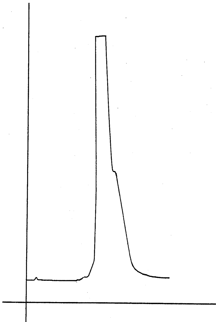
GLC PROFILE FOR EXAMPLE II, DIISOUNDECANAL.
