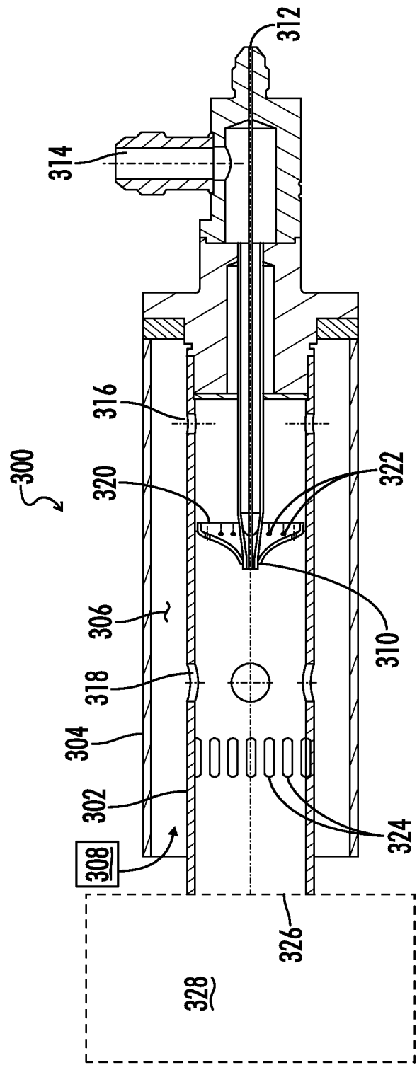
FIG. 9 (PRIOR ART)
