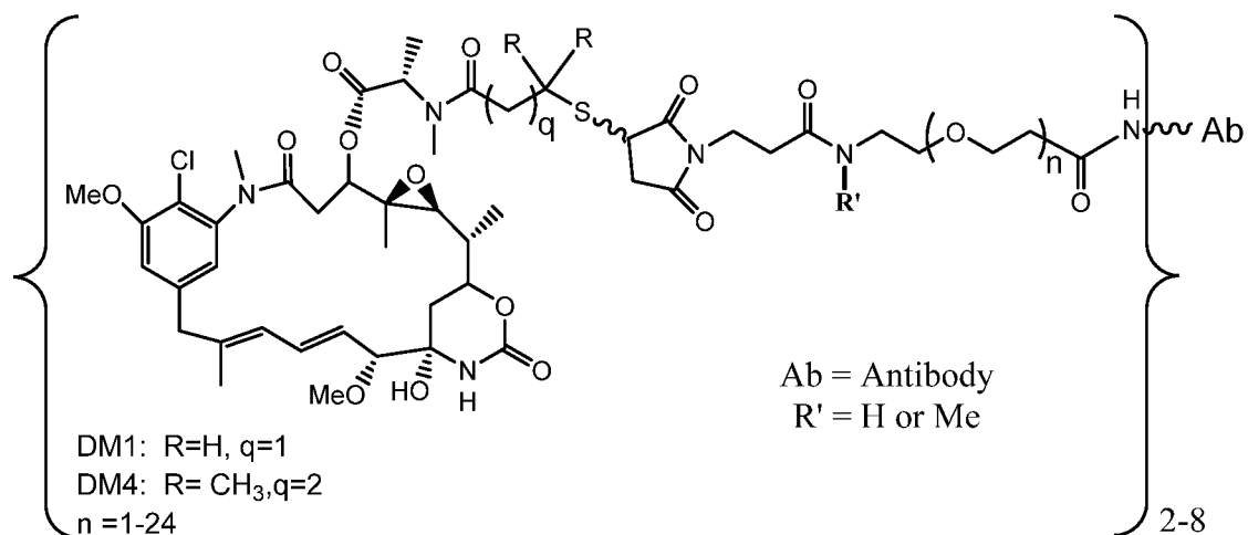
Ab-PEG-Mal-DM1/DM4
