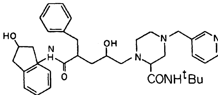
FIG. 1C Indinavir (L-735,524)
