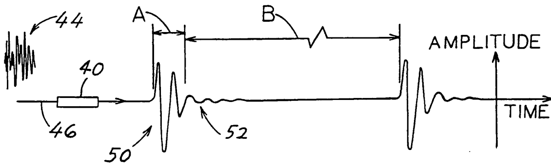
FIG. 2 TRANSMITTED PULSE
