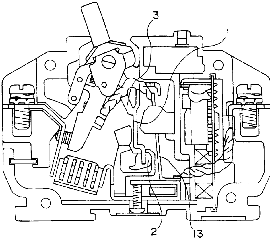
FIG. 8 (PRIOR ART)
