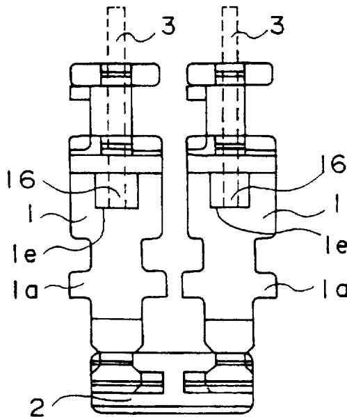
FIG. 9 (PRIOR ART)
