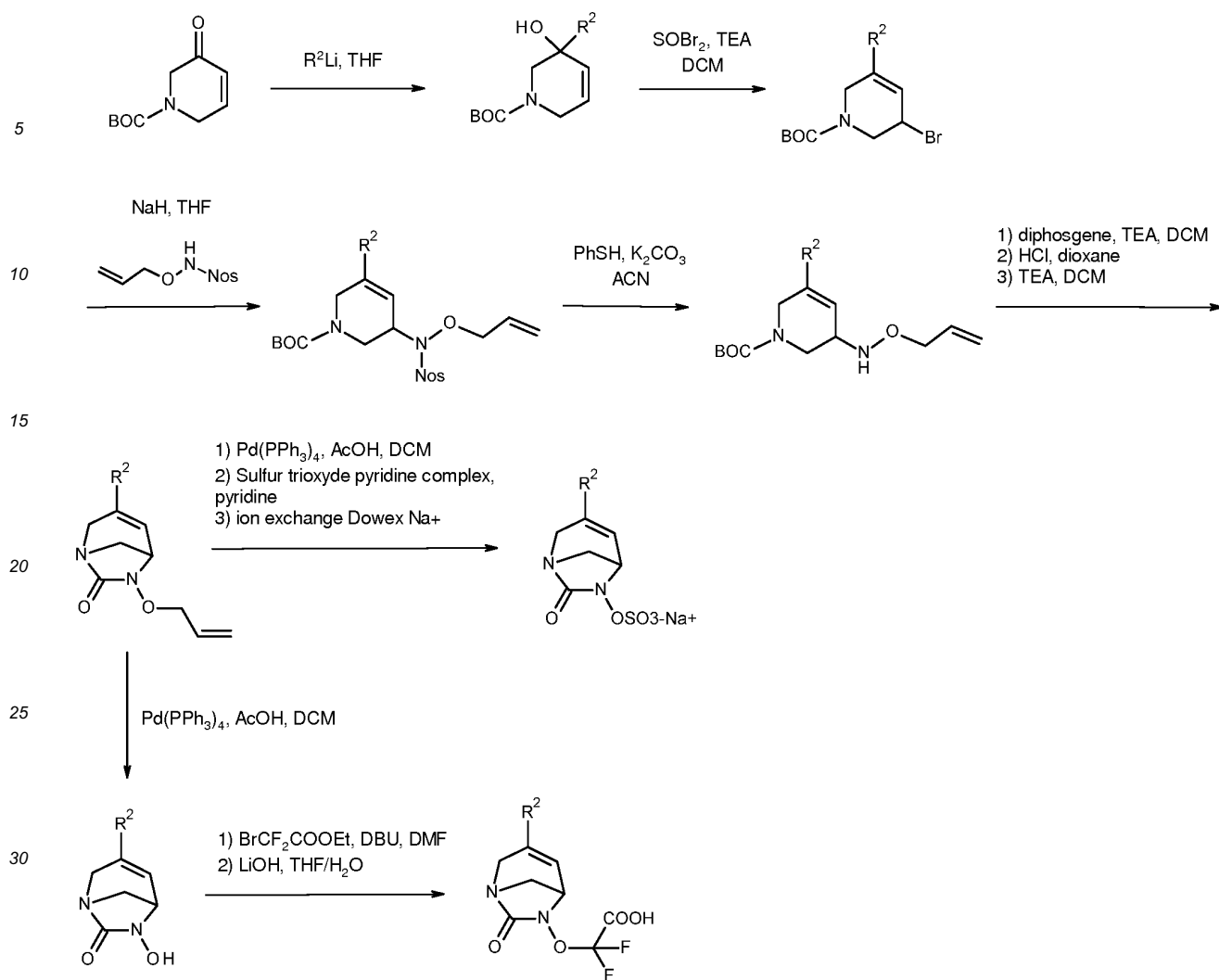
Scheme 4
