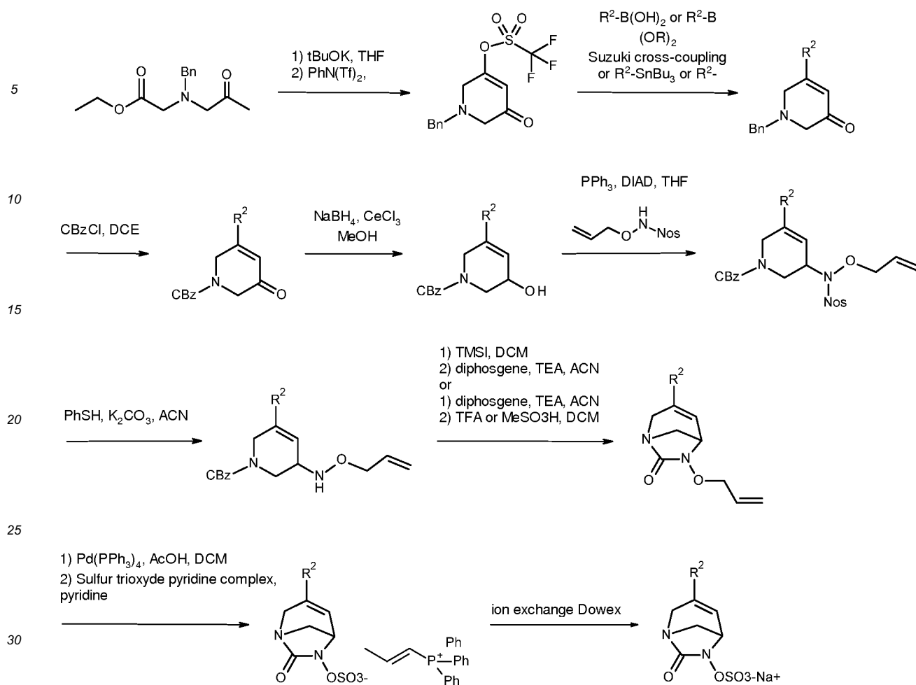
Scheme 2
