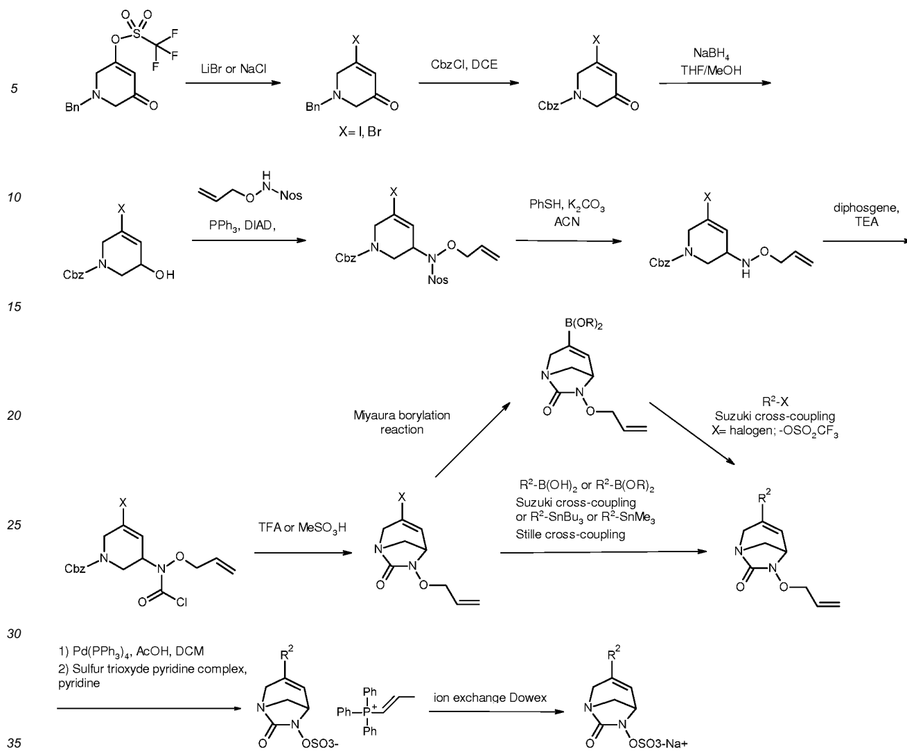
Scheme 3
