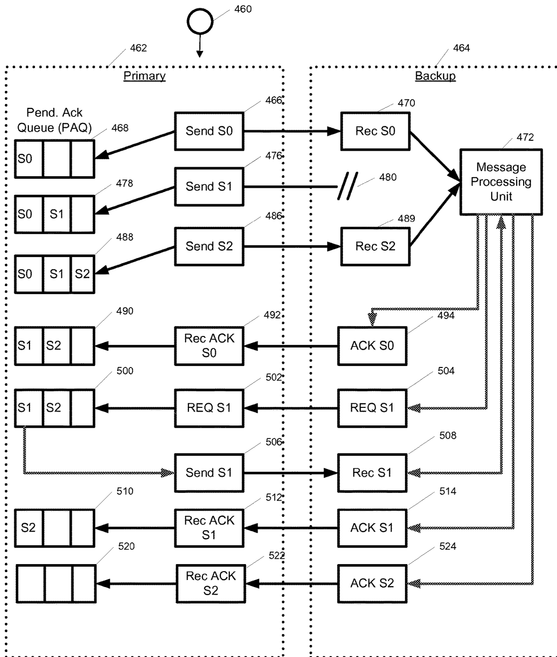
Fig.12 – Multiple message with Retransmit
