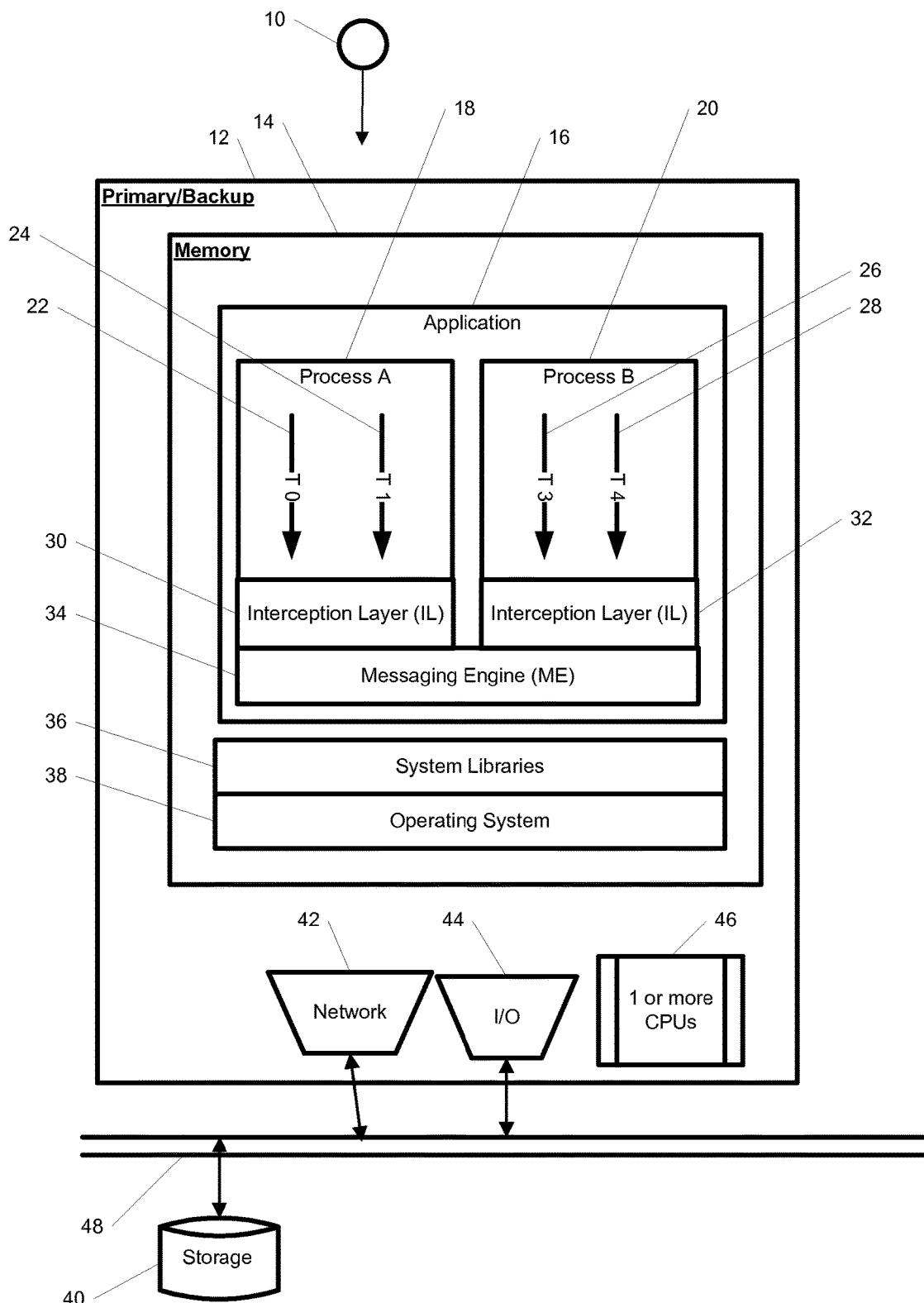
FIG.1 – Primary and Backup Architecture
