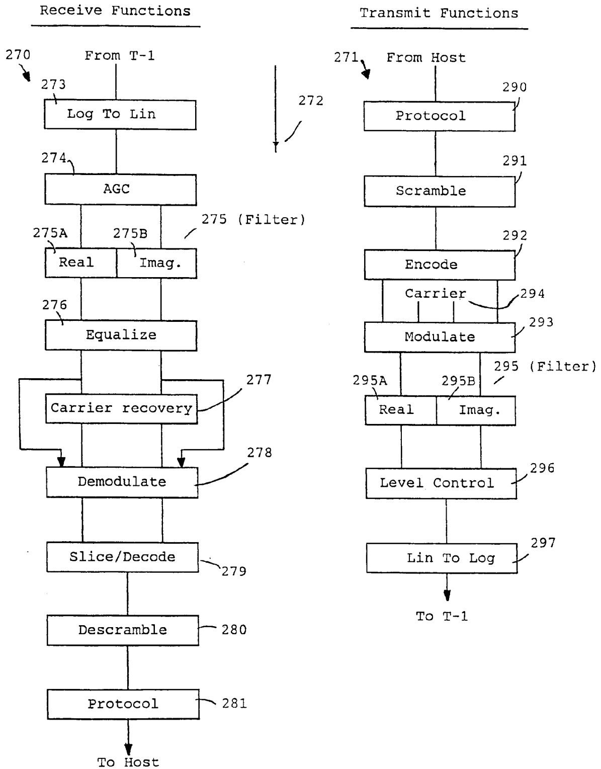
Fig. 15 (Example of Coherent Phase Shift Keyed Modem)
