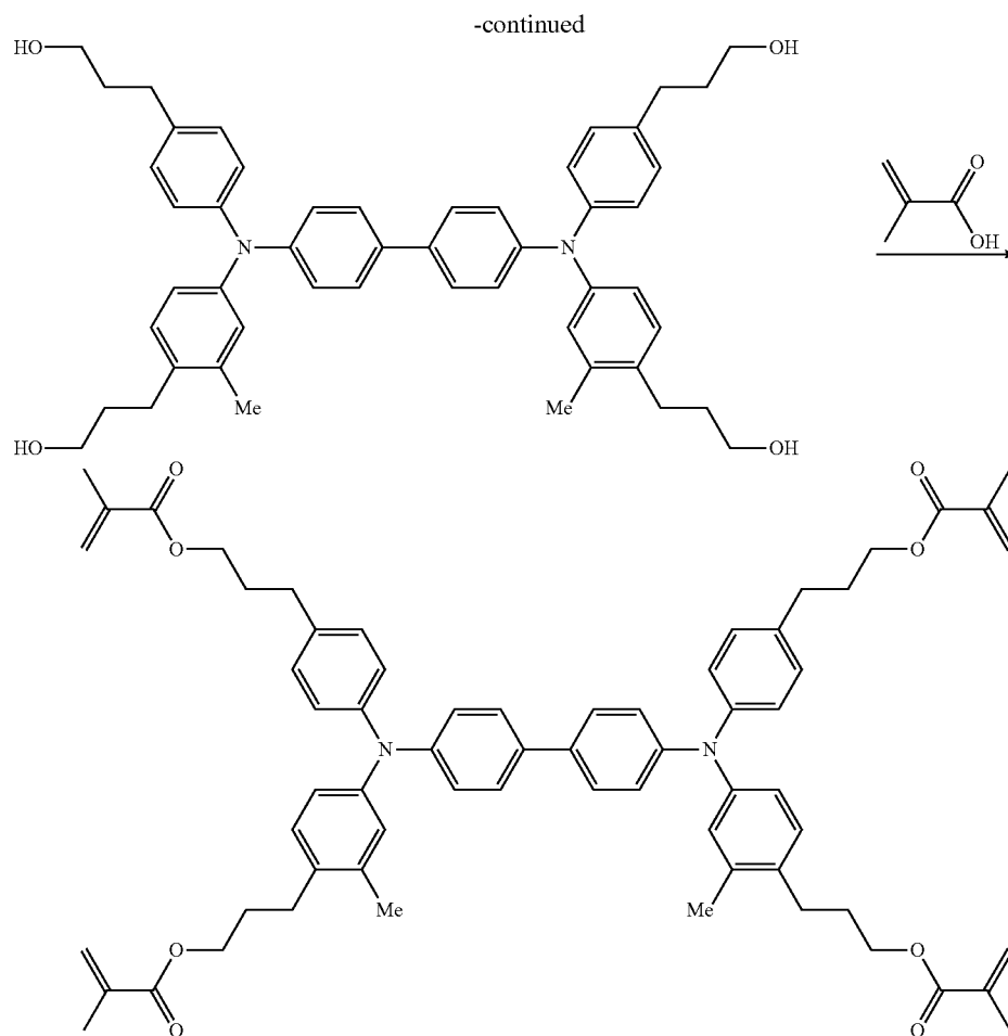
Compound iv-17
