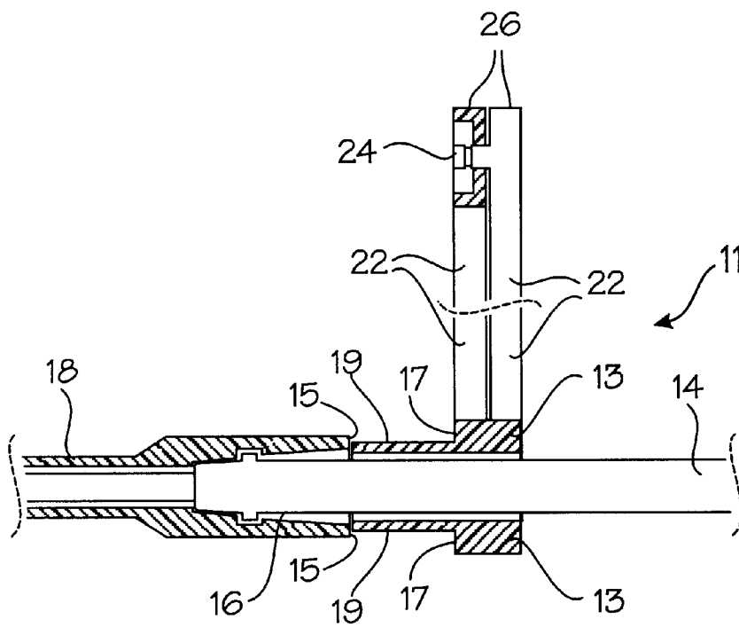
Fig. 2 (Prior Art)
