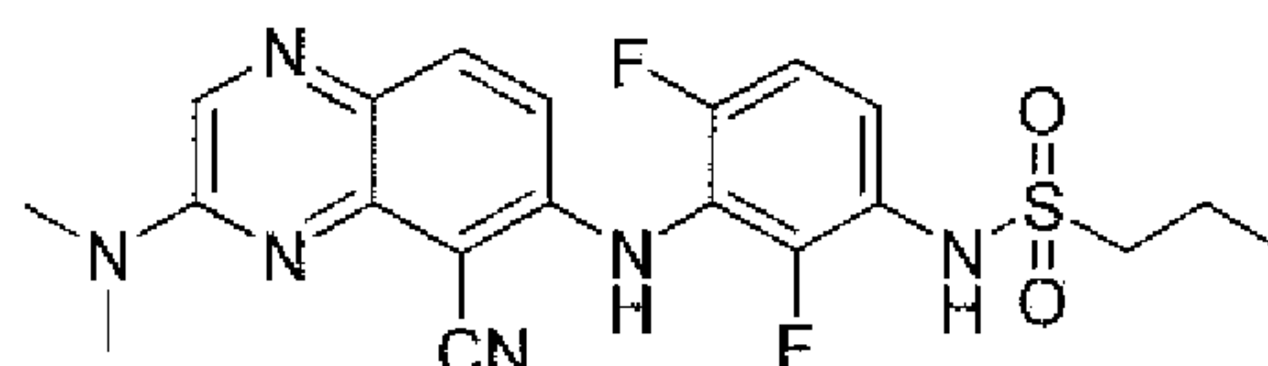
N -(3-(5-cyano-3-(dimethylamino)quinoxalin-6-ylamino)-2,4-difluorophenyl)propane-1-sulfonamide
