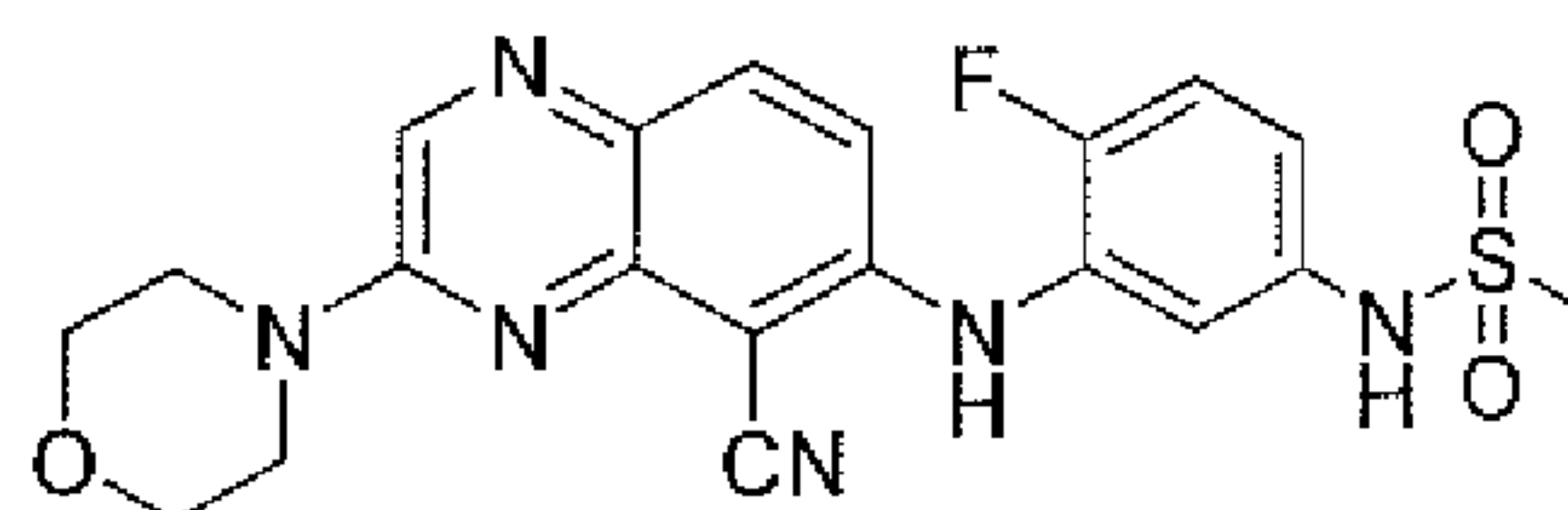
N -(3-(5-cyano-3-morpholinoquinoxalin-6-ylamino)-4-fluorophenyl)methanesulfonamide
