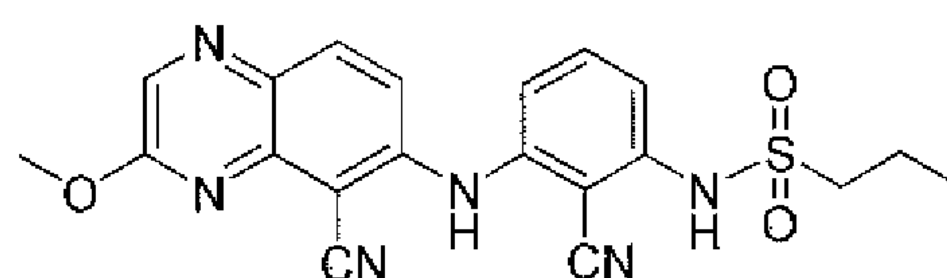
N -(2-cyano-3-(5-cyano-3-methoxyquinoxalin-6-ylamino)phenyl)propane-1-sulfonamide
