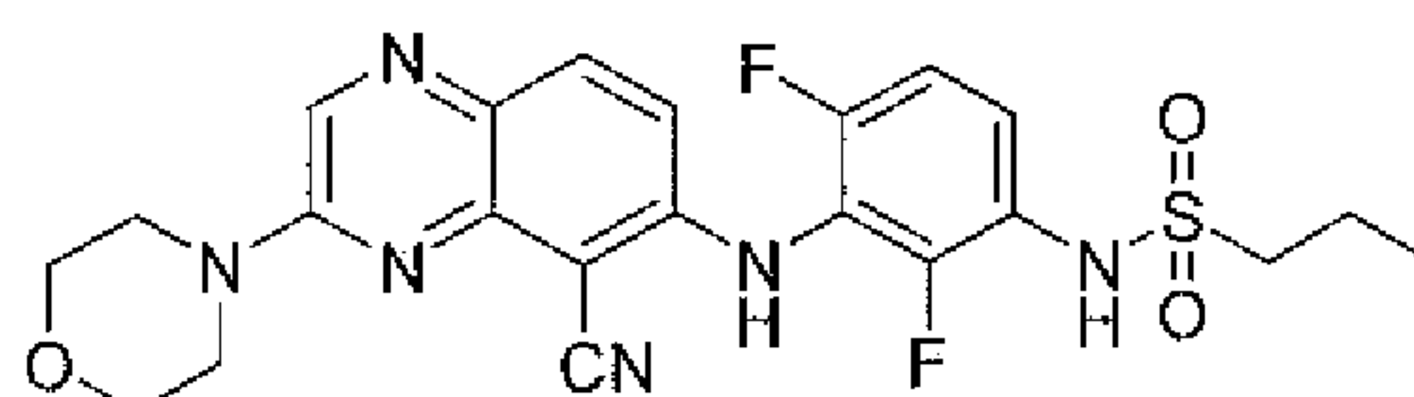
N -(3-(5-cyano-3-morpholinoquinoxalin-6-ylamino)-2,4-difluorophenyl)propane-1-sulfonamide
