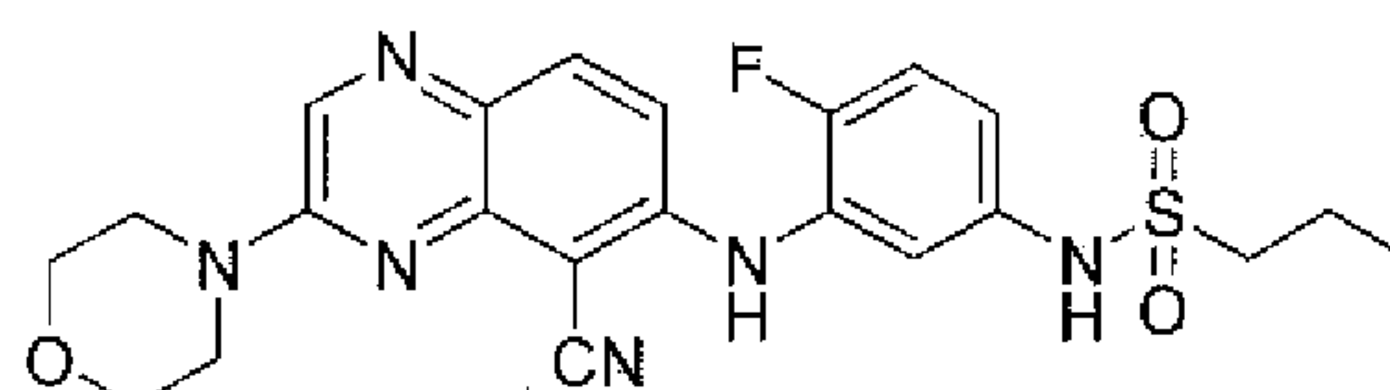
N -(3-(5-cyano-3-morpholinoquinoxalin-6-ylamino)-4-fluorophenyl)propane-1-sulfonamide
