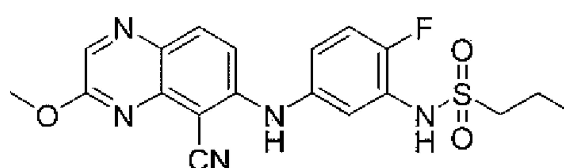
N -(5-(5-cyano-3-methoxyquinoxalin-6-ylamino)-2-fluorophenyl)propane-1-sulfonamide
