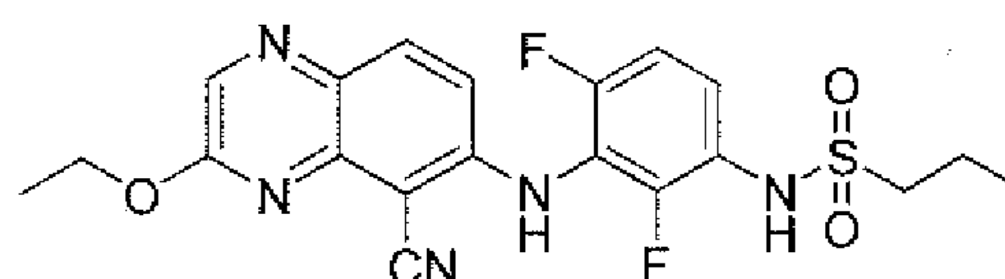
N-(3-(5-cyano-3-ethoxyquinolaliny)-2,4-difluorophenyl)propane-1-sulfonamide
