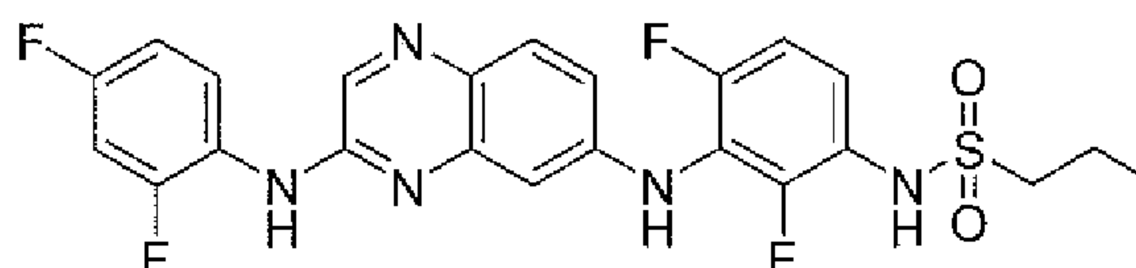
N1-(3-([3-(2,4-difluoroanilino)-6-quinolaliny]amino)-2,4-difluorophenyl)-1-propanesulfonamide
