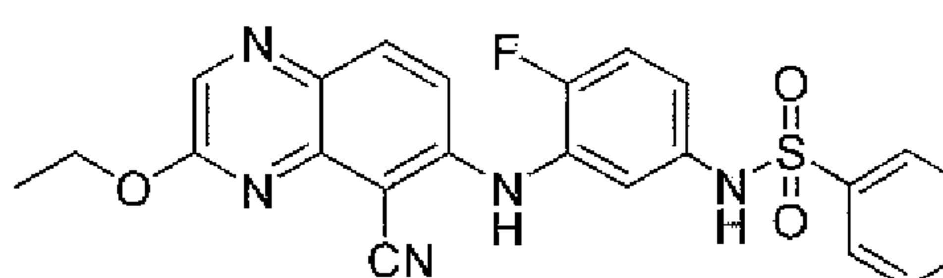
N -(3-(5-cyano-3-ethoxyquinoxalin-6-ylamino)-4-fluorophenyl)benzenesulfonamide
