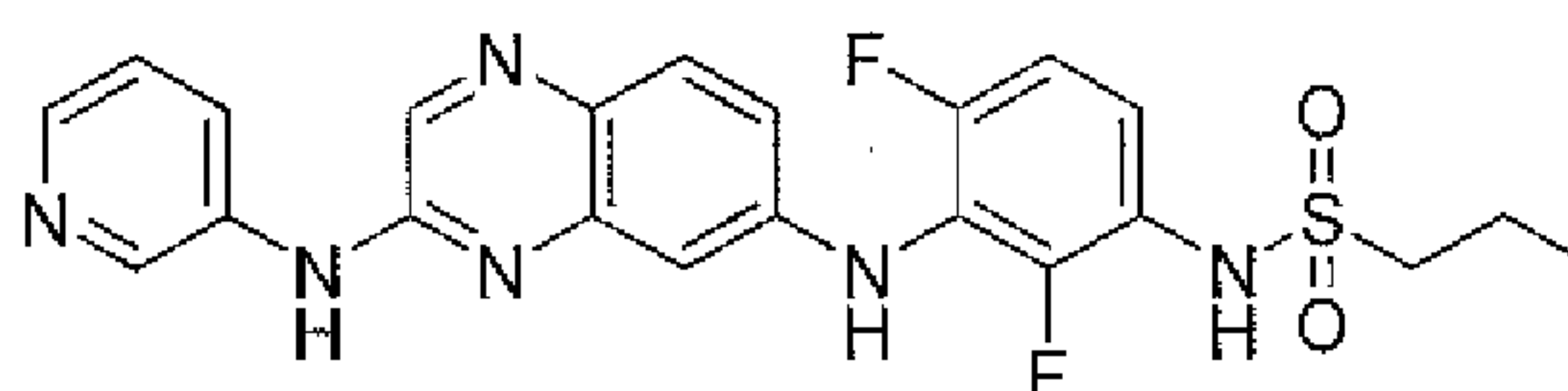
N1-(2,4-difluoro-3-([3-(3-pyridylamino)-6-quinolaliny]amino)phenyl)-1-propanesulfonamide
