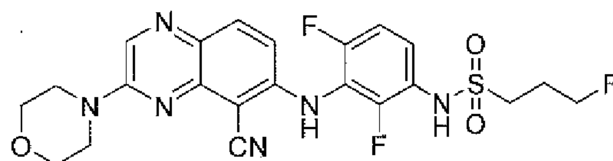
N -(3-(5-cyano-3-morpholinoquinoxalin-6-ylamino)-2,4-difluorophenyl)-3-fluoropropane-1-sulfonamide
