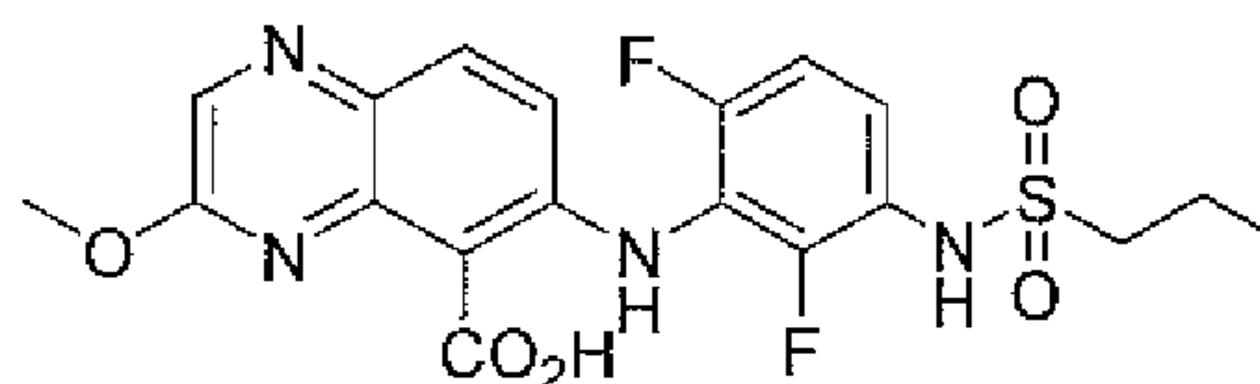
6-(2,6-difluoro-3-(propylsulfonamido)phenylamino)-3-methoxyquinoxaline-5-carboxylic acid
