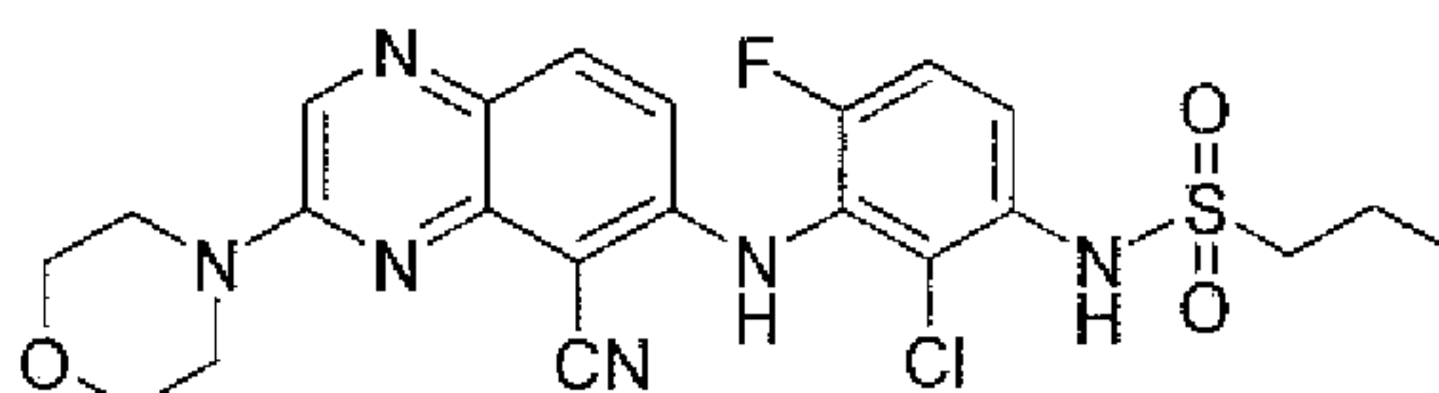
N -(2-chloro-3-(5-cyano-3-morpholinoquinoxalin-6-ylamino)-4-fluorophenyl)propane-1-sulfonamide
