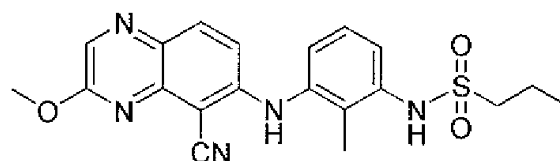
N -(3-(5-cyano-3-methoxyquinoxalin-6-ylamino)-2-methylphenyl)propane-1-sulfonamide
