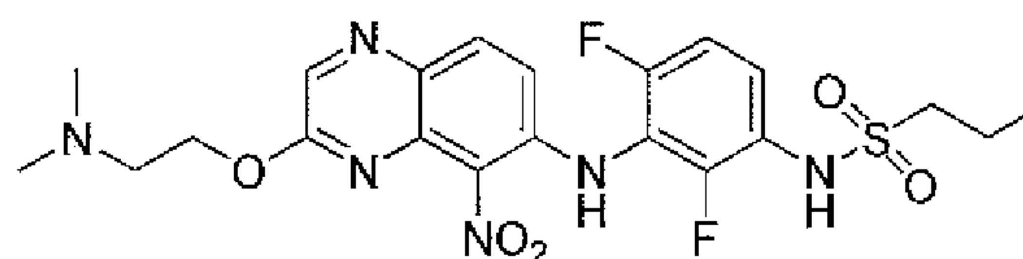
N1-[3-[(3-[2-(dimethylamino)ethoxy]-5-nitro-6-quinoxaliny)amino]-2,4-difluorophenyl]-1-propanesulfonamide
