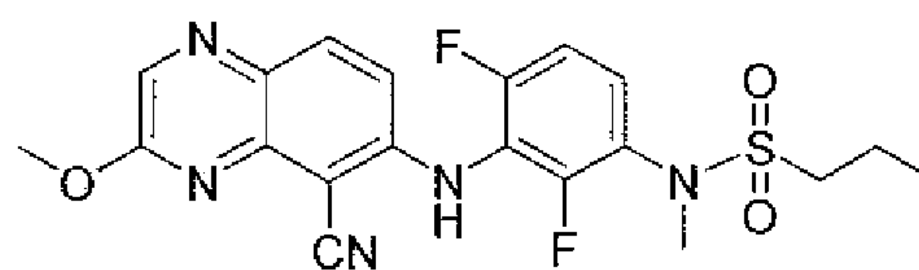
N -(3-(5-cyano-3-methoxyquinoxalin-6-ylamino)-2,4-difluorophenyl)- N -methylpropane-1-sulfonamide
