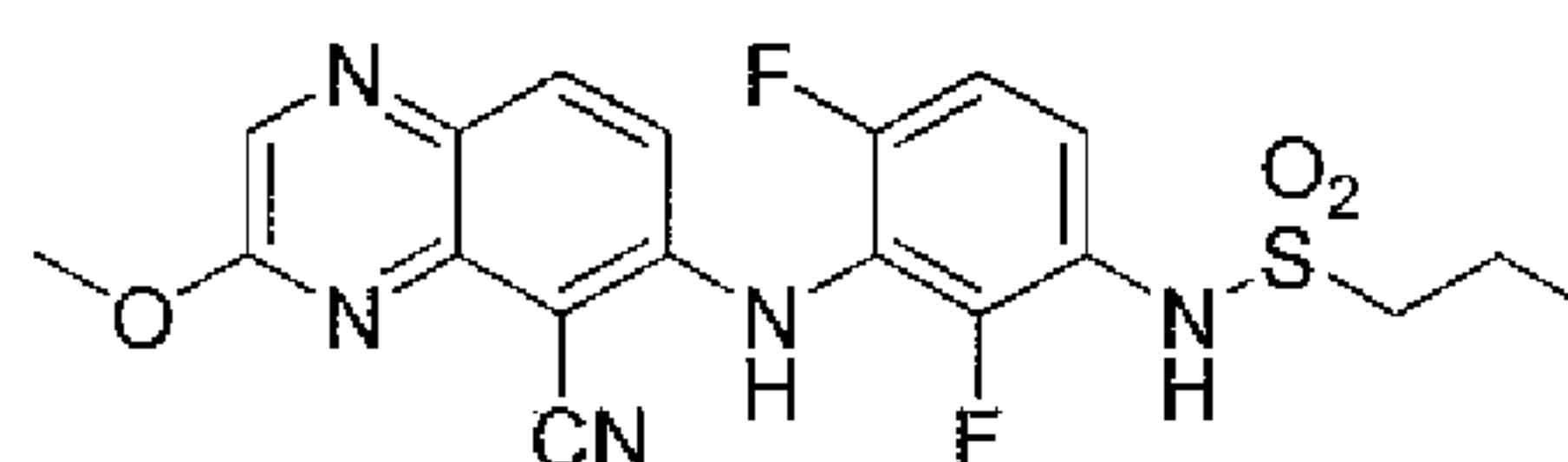
N1-[3-[(5-cyano-3-methoxy-6-quinoxaliny)amino]-2,4-difluorophenyl]-1-propanesulfonamide
