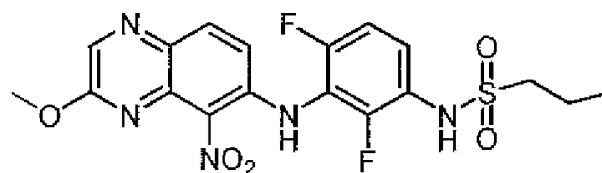
N1-(2,4-difluoro-3-[(3-methoxy-5-nitro-6-quinoxaliny)amino]phenyl)-1-propanesulfonamide
