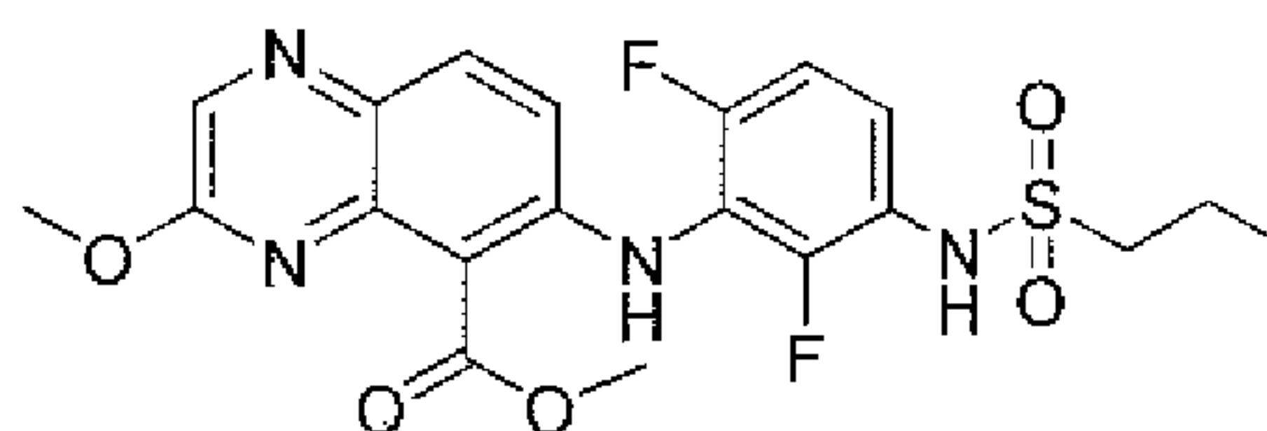
methyl 6-(2,6-difluoro-3-(propylsulfonamido)phenylamino)-3-methoxyquinoxaline-5-carboxylate
