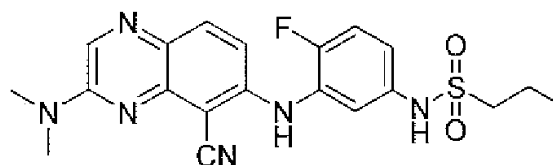
N -(3-(5-cyano-3-(dimethylamino)quinoxalin-6-ylamino)-4-fluorophenyl)propane-1-sulfonamide
