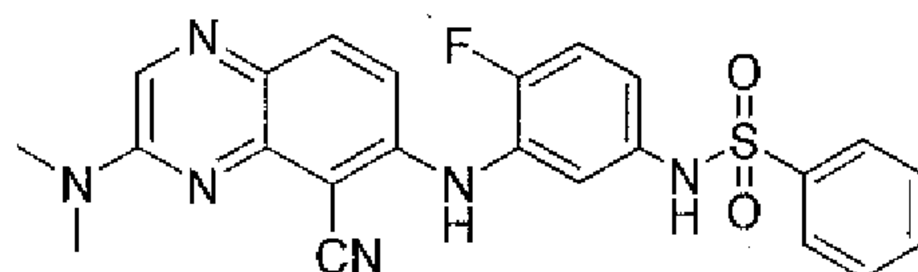
N -(3-(5-cyano-3-(dimethylamino)quinoxalin-6-ylamino)-4-fluorophenyl)benzenesulfonamide
