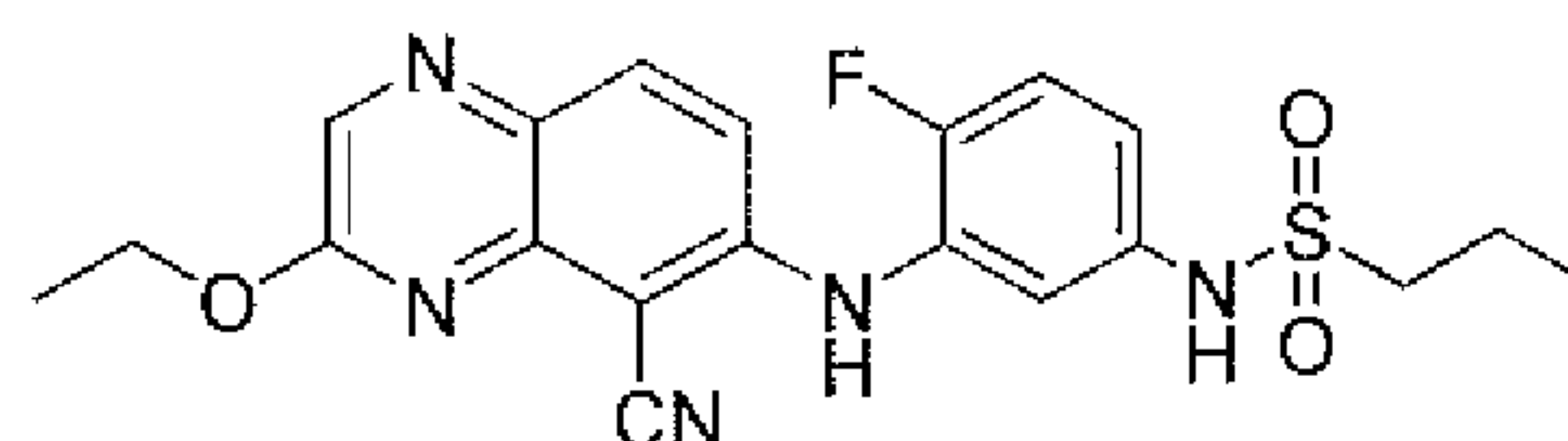
N -(3-(5-cyano-3-ethoxyquinoxalin-6-ylamino)-4-fluorophenyl)propane-1-sulfonamide
