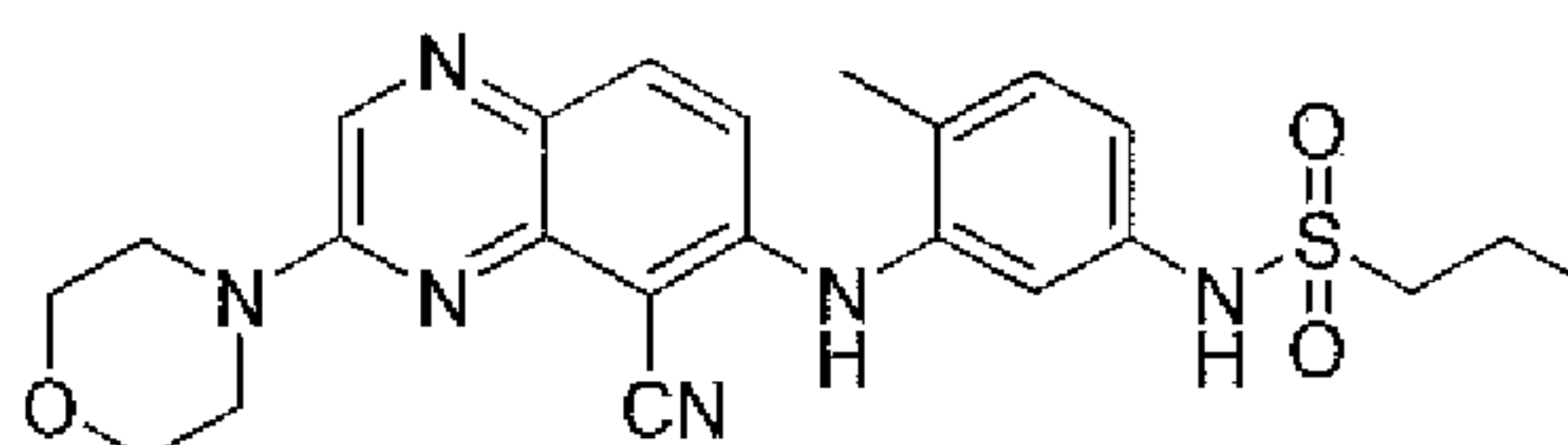
N -(3-(5-cyano-3-morpholinoquinoxalin-6-ylamino)-4-methylphenyl)propane-1-sulfonamide
