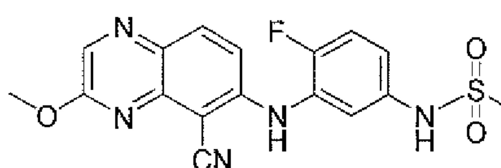
N -(3-(5-cyano-3-methoxyquinoxalin-6-ylamino)-4-fluorophenyl)methanesulfonamide
