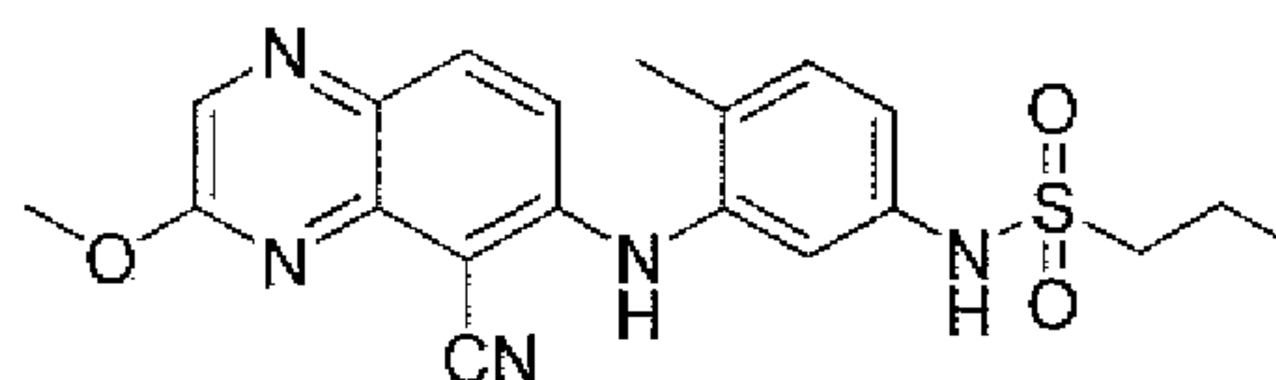
N -(3-(5-cyano-3-methoxyquinoxalin-6-ylamino)-4-methylphenyl)propane-1-sulfonamide
