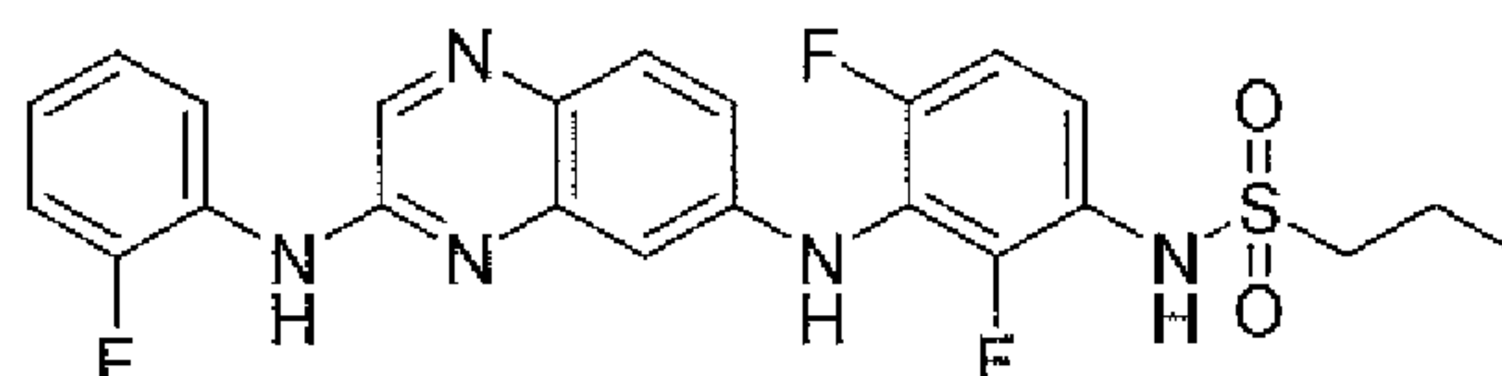
N1-(2,4-difluoro-3-([3-(2-fluoroanilino)-6-quinolaliny]amino)phenyl)-1-propanesulfonamide
