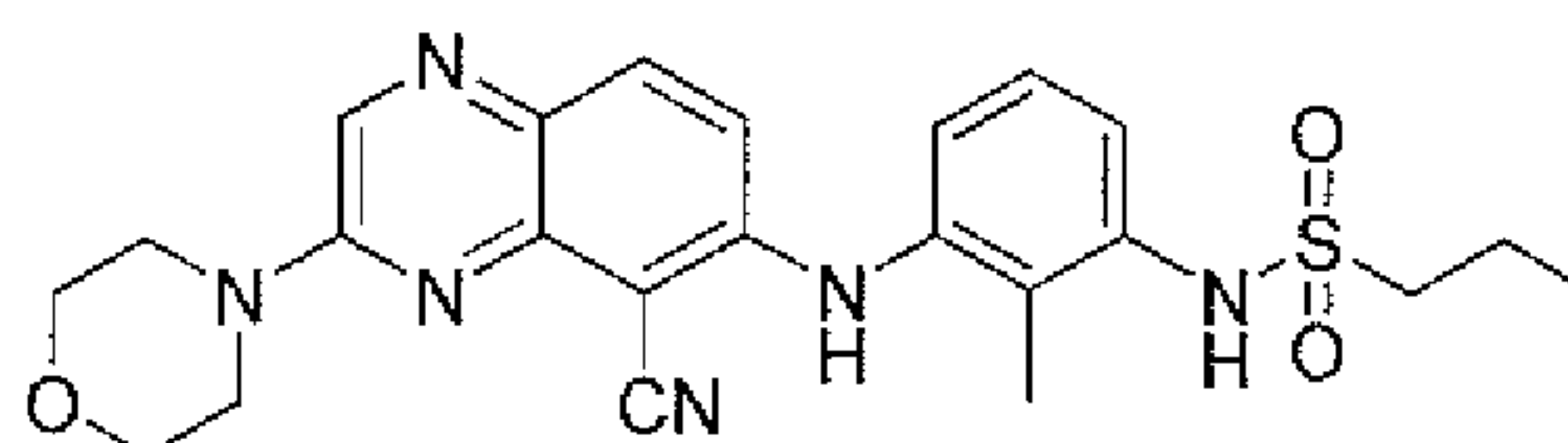
N -(3-(5-cyano-3-morpholinoquinoxalin-6-ylamino)-2-methylphenyl)propane-1-sulfonamide
