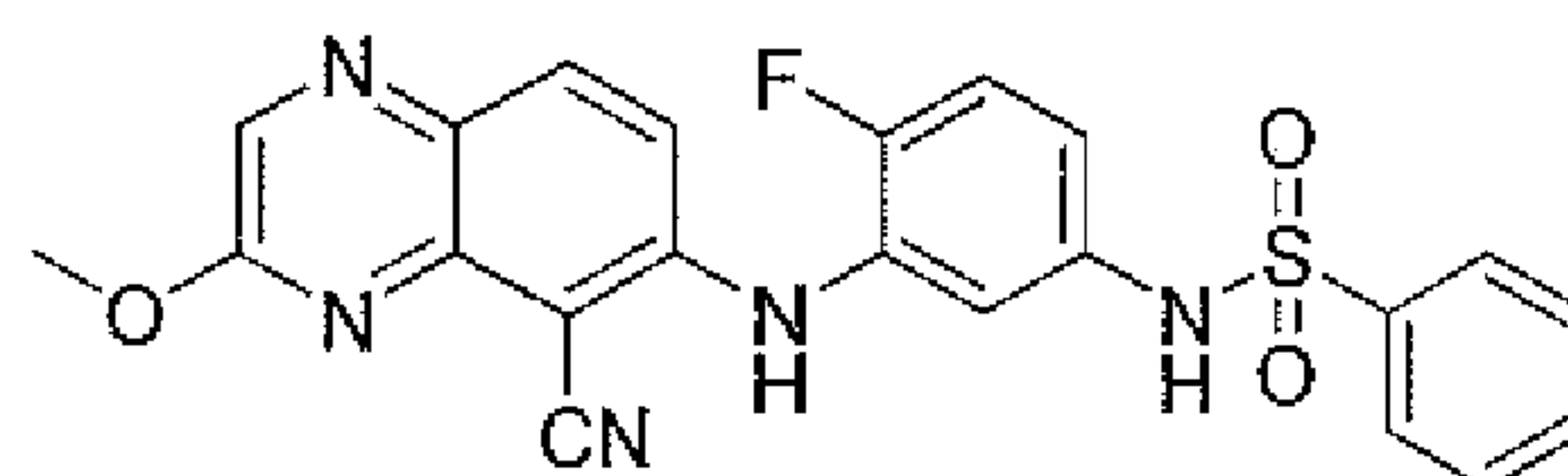
N -(3-(5-cyano-3-methoxyquinoxalin-6-ylamino)-4-fluorophenyl)benzenesulfonamide
