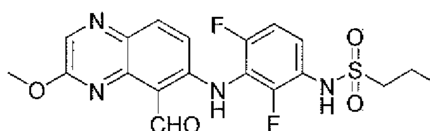
N -(2,4-difluoro-3-(5-formyl-3-methoxyquinoxalin-6-ylamino)phenyl)propane-1-sulfonamide
