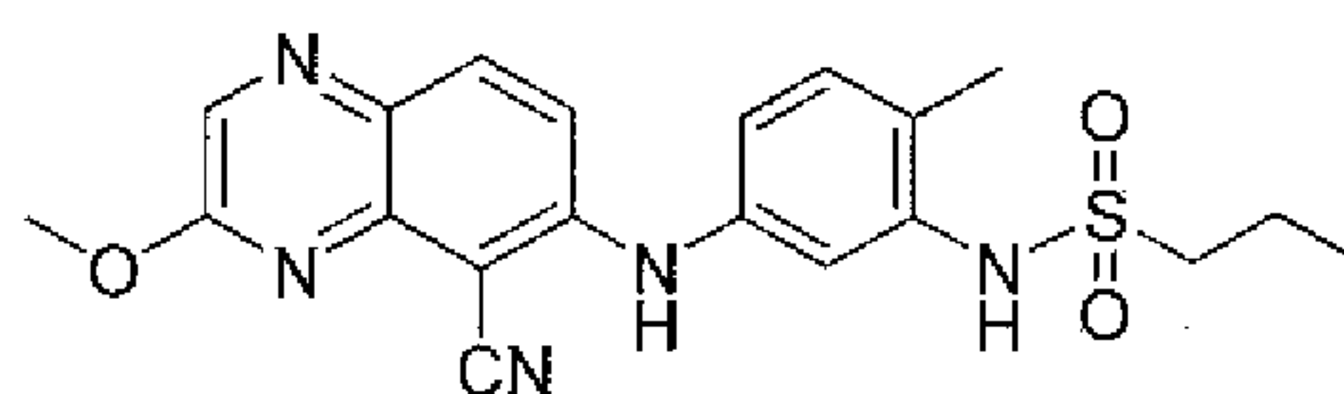
N -(5-(5-cyano-3-methoxyquinoxalin-6-ylamino)-2-methylphenyl)propane-1-sulfonamide
