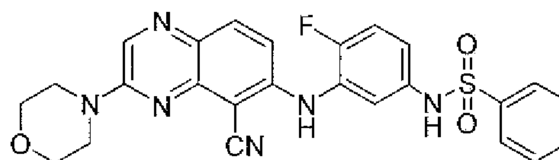
N -(3-(5-cyano-3-morpholinoquinoxalin-6-ylamino)-4-fluorophenyl)benzenesulfonamide
