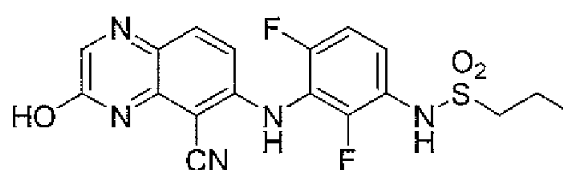
N1-(3-([5-cyano-3-hydroxy-6-quinolaliny]amino)-2,4-difluorophenyl)-1-propanesulfonamide
