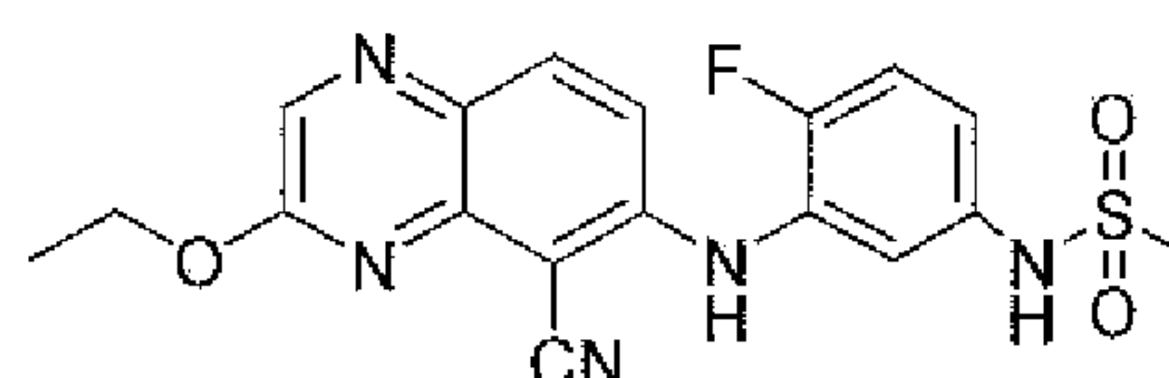
N -(3-(5-cyano-3-ethoxyquinoxalin-6-ylamino)-4-fluorophenyl)methanesulfonamide
