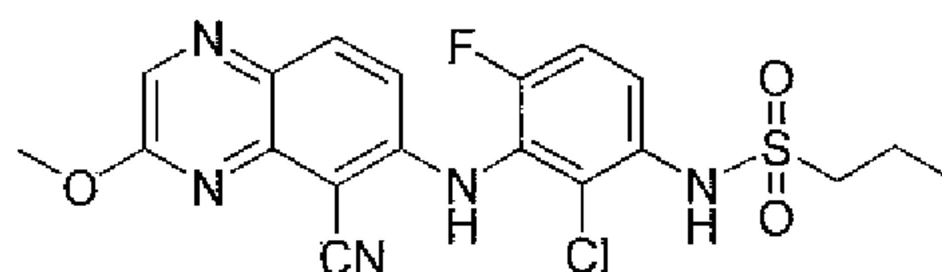
N -(2-chloro-3-(5-cyano-3-methoxyquinoxalin-6-ylamino)-4-fluorophenyl)propane-1-sulfonamide
