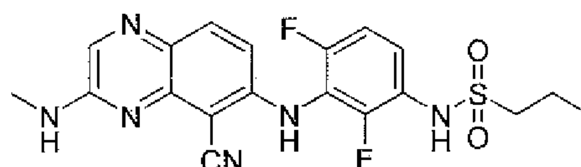
N -(3-(5-cyano-3-(methylamino)quinoxalin-6-ylamino)-2,4-difluorophenyl)propane-1-sulfonamide
