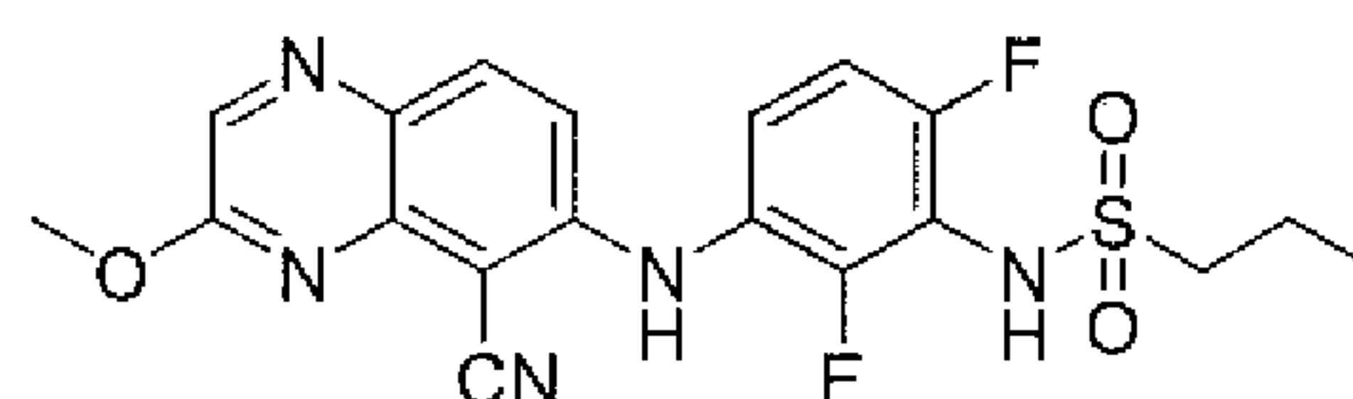
N -(3-(5-cyano-3-methoxyquinoxalin-6-ylamino)-2,6-difluorophenyl)propane-1-sulfonamide
