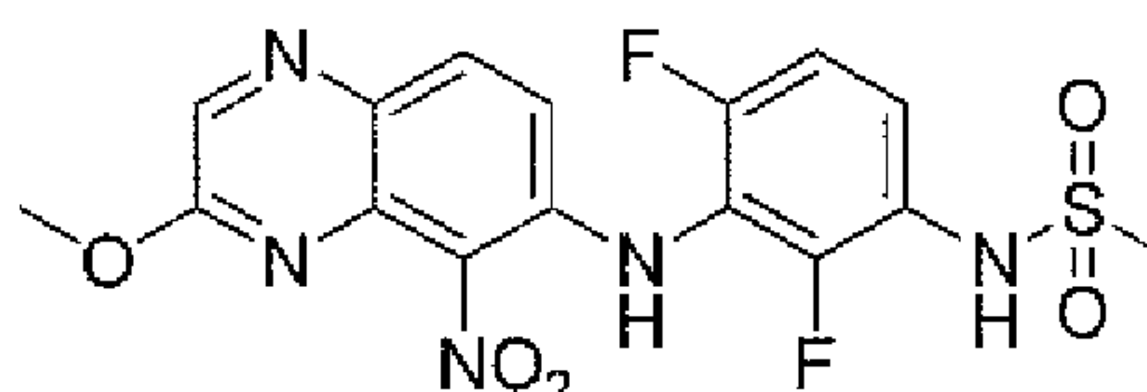
N-[2,4-difluoro-3-([3-methoxy-5-nitro-6-quinolaliny]amino)phenyl]methanesulfonamide
