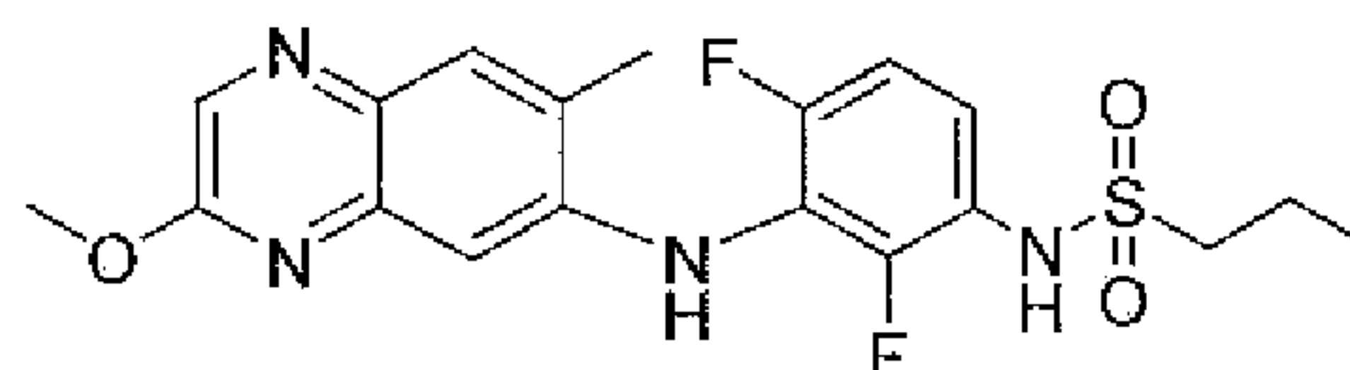
N -(2,4-difluoro-3-(3-methoxy-7-methylquinoxalin-6-ylamino)phenyl)propane-1-sulfonamide
