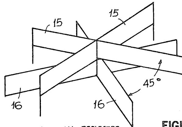
OMNIDIRECTIONAL REFLECTOR
