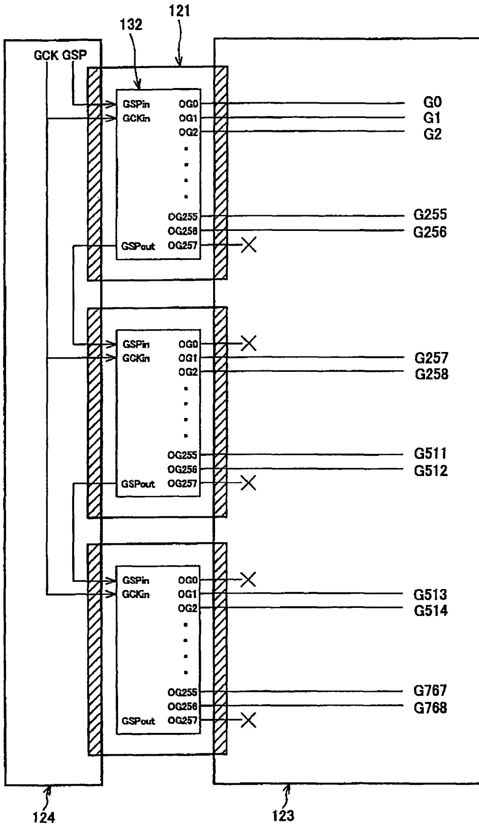
FIG. 29 (PRIOR ART)
