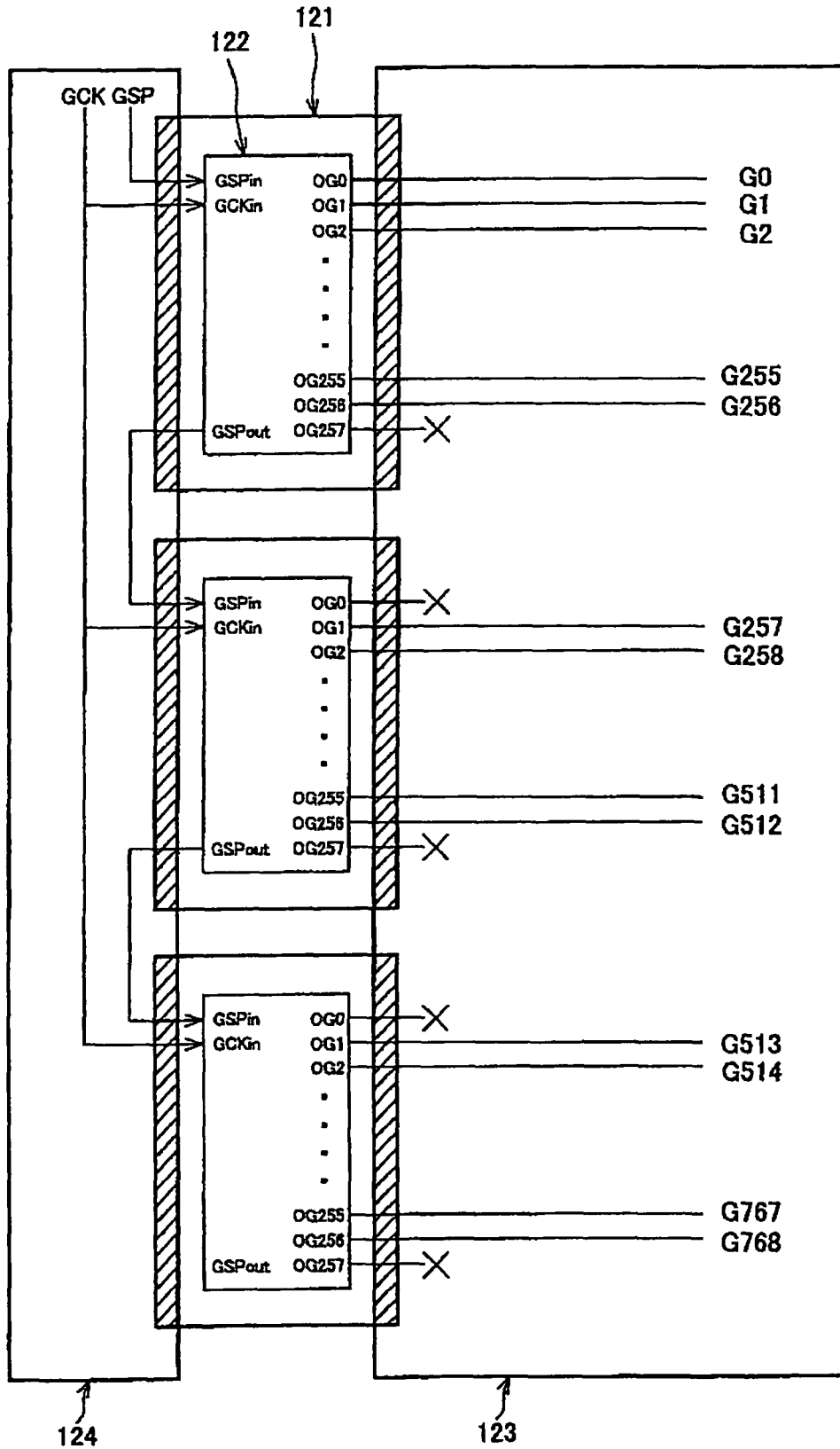
FIG. 23 (PRIOR ART)
