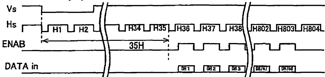
FIG. 26 (c) (PRIOR ART)
