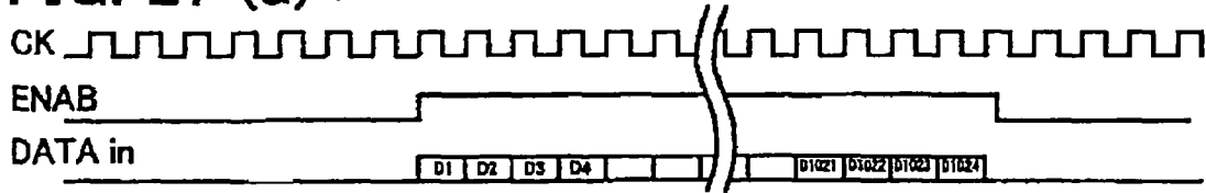
FIG. 27 (b) (PRIOR ART)
