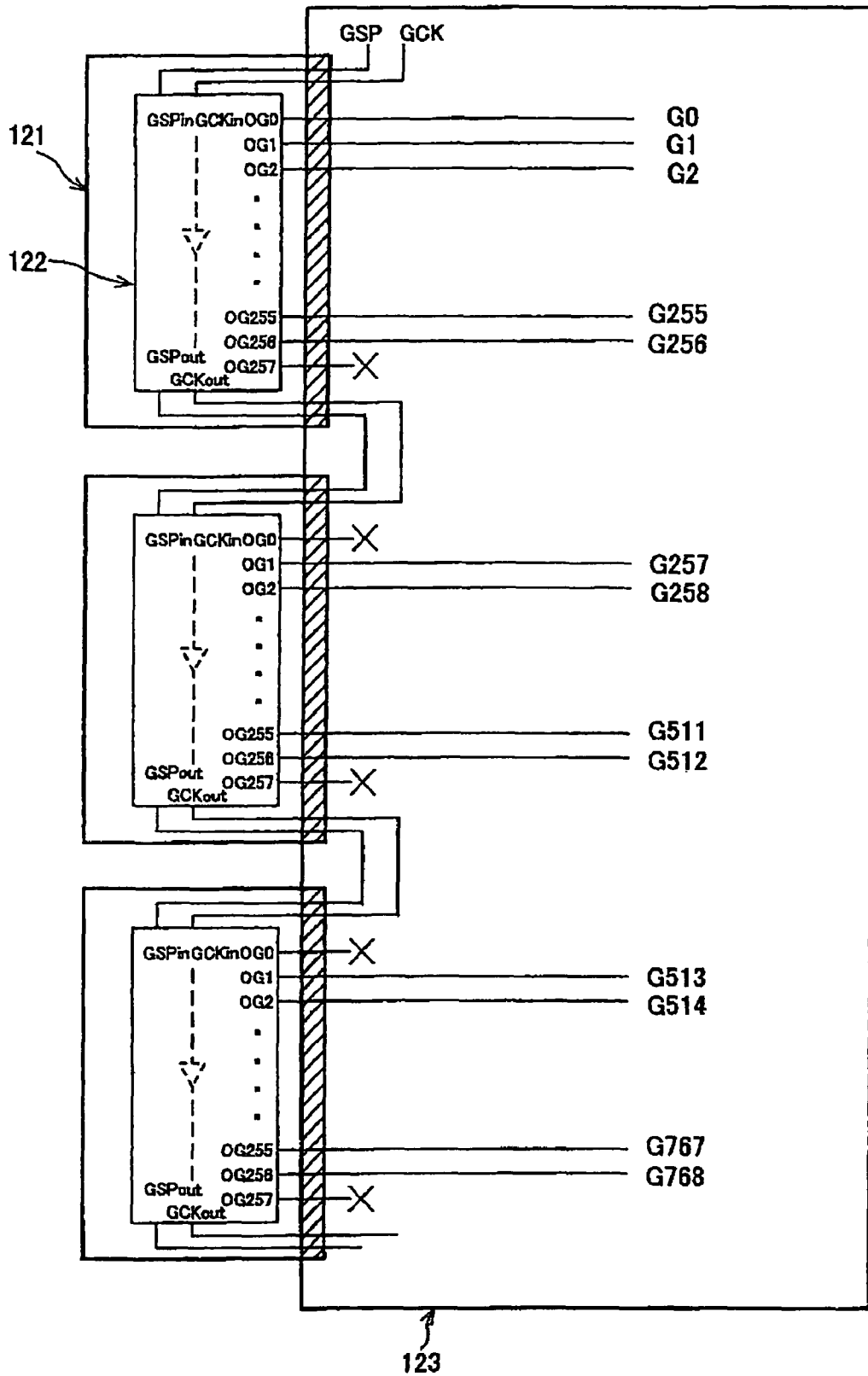
FIG. 25 (PRIOR ART)
