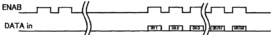
FIG. 27 (c) (PRIOR ART)
