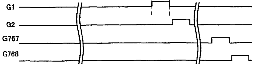
FIG. 26 (f) (PRIOR ART)
