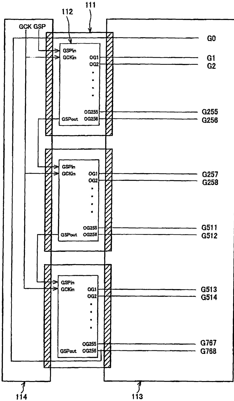
FIG. 21 (PRIOR ART)
