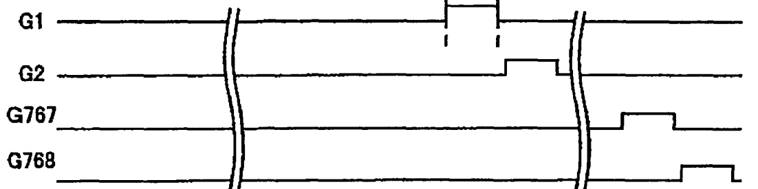
FIG. 27 (f) (PRIOR ART)
