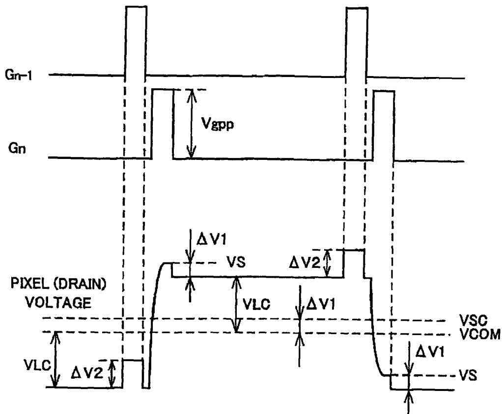
FIG. 20 (PRIOR ART)
