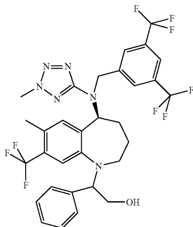
Example 88
