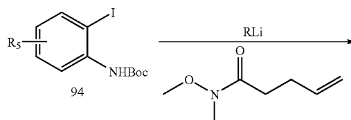
Scheme 15
