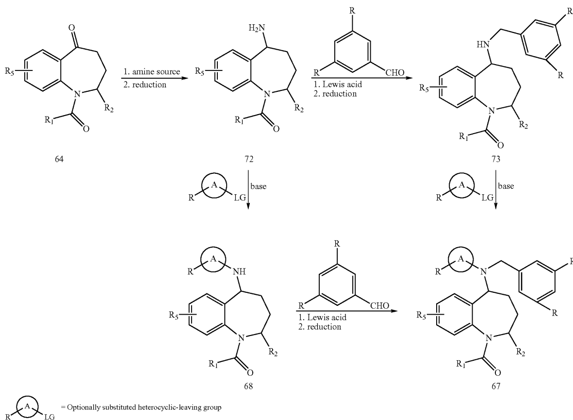
Scheme 9
