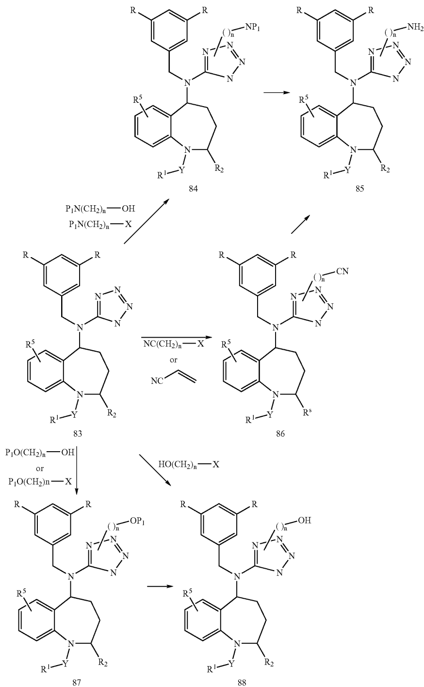
Scheme 12
