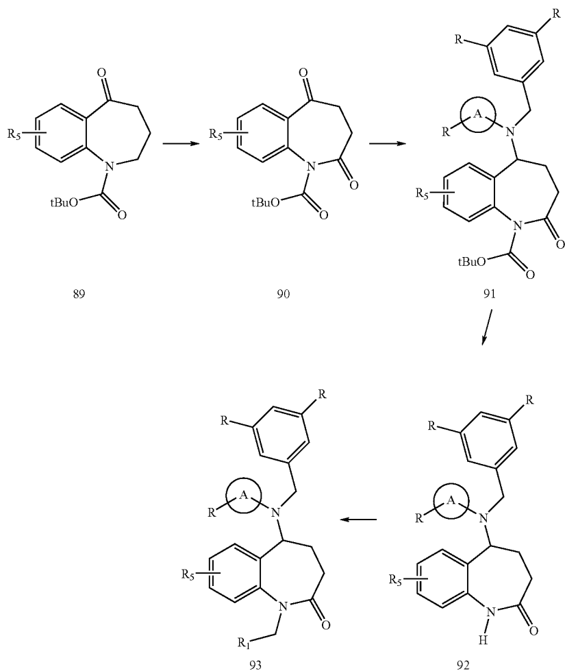
Scheme 14
