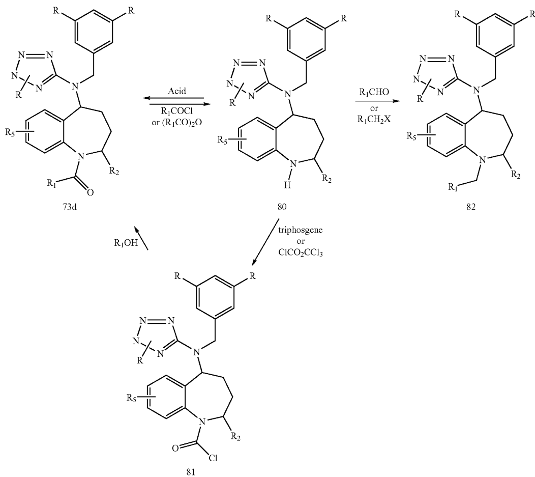
Scheme 11
