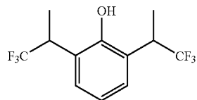
2,6-Bis-(2,2,2-trifluoro-1-methyl-ethyl)-phenol
