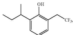
2-sec-Butyl-6-(2,2,2-trifluoro-ethyl)-phenol
