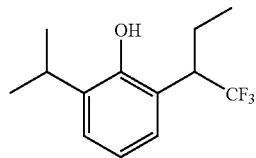
2-Isopropyl-6-(1-trifluoromethyl-propyl)-phenol
