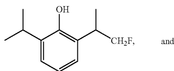
2-(2-Fluoro-1-methyl-ethyl)-6-isopropyl-phenol
