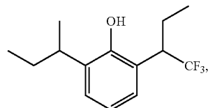
2-sec-Butyl-6-(1-trifluoromethyl-propyl)-phenol
