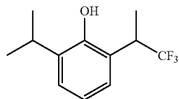
2-Isopropyl-6-(2,2,2-trifluoro-1-methyl-ethyl)-phenol
