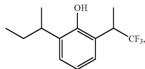
2-sec-Butyl-6-(2,2,2-trifluoro-1-methyl-ethyl)-phenol
