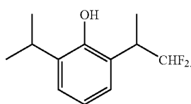
2-(2,2,-Difluoro-1-methyl-ethyl)-6-isopropyl-phenol
