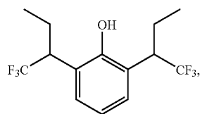
2,6-Bis-(1-trifluoromethyl-propyl)-phenol
