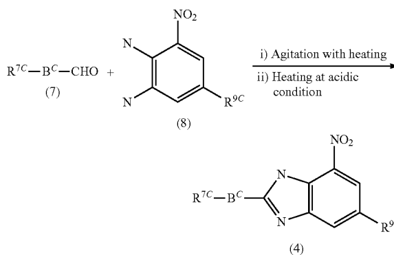
Reaction Scheme 2
