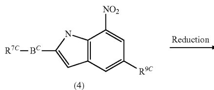
Reaction Scheme 1
