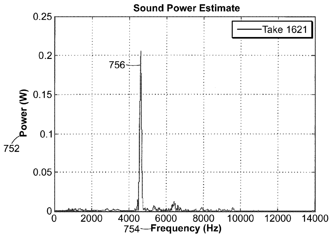
FIG. 7 (Prior Art)
