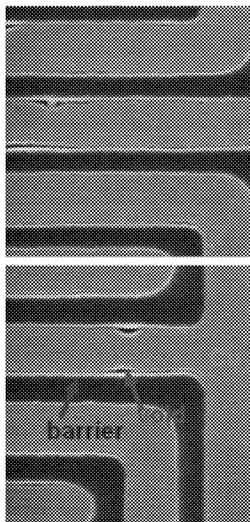
FIG. 1C (PRIOR ART)
