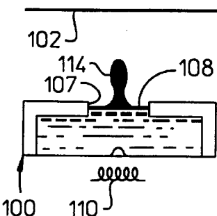
(PRIOR ART) FIG. 1C
