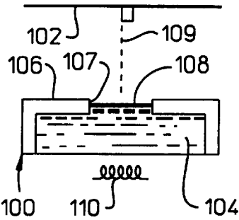
(PRIOR ART) FIG. 1A
