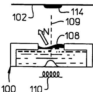
(PRIOR ART) FIG. 1F
