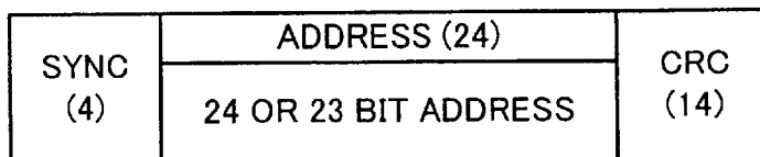
ATIP FORMAT OF HIGH DENSITY DISC
