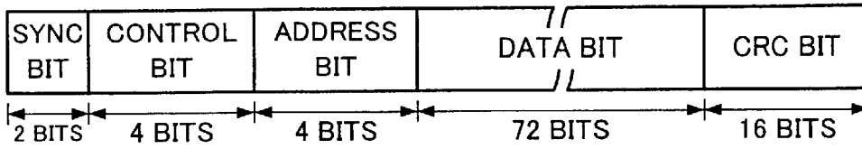
FORMAT OF Q CHANNEL
