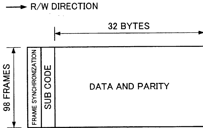
FORMAT OF SUB CODE FRAME OF CD
