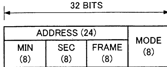
FORMAT OF HEADER PORTION OF CONVENTIONAL CD-ROM
