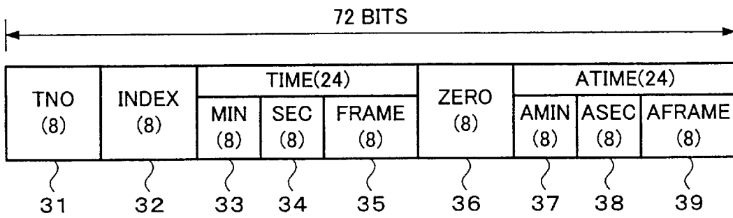
FORMAT OF DATA BIT BLOCK
