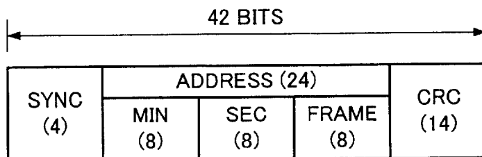
ATIP FORMAT OF CONVENTIONAL DISC
