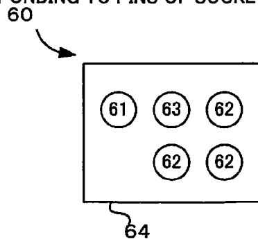
(b) TOP VIEW OF PRINTED WIRING BOARD WITH THROUGH HOLES CORRESPONDING TO PINS OF SOCKETS ARRANGED WITH 2.54 mm PITCH
