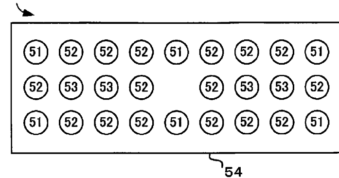
(a) TOP VIEW OF PRINTED WIRING BOARD WITH THROUGH HOLES CORRESPONDING TO PINS OF CONNECTORS ARRANGED WITH 2.54 mm PITCH
