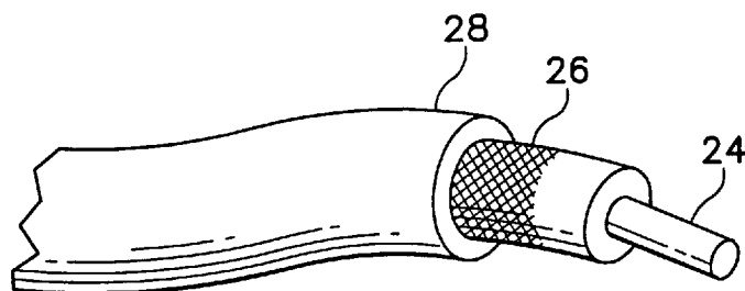
FIG. 2 (PRIOR ART)
