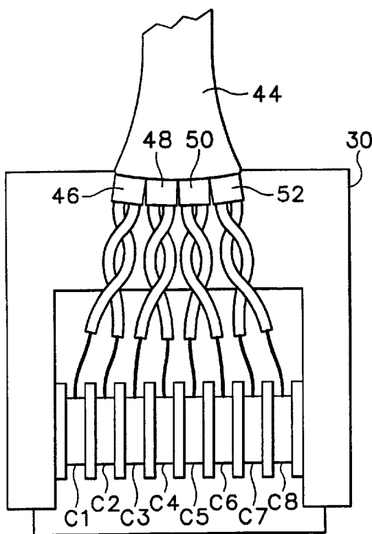
FIG. 4 (PRIOR ART)
