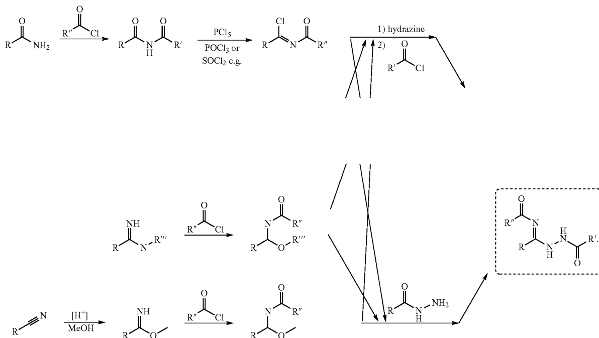
Scheme V:
