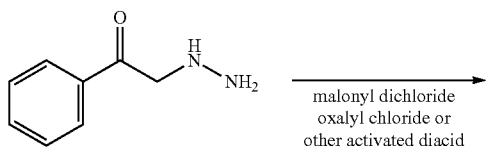
Scheme XII.
